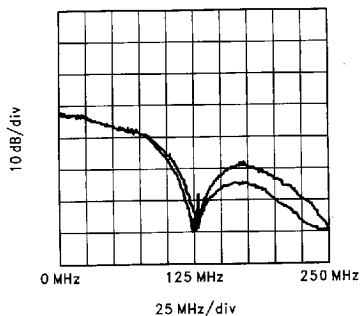
FIGURE 5. 1V Binary Power Spectrum with and without Edge Rate Control
