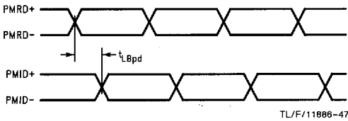
FIGURE 31. PMID Timing (Loopback)
