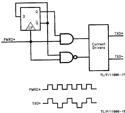
FIGURE 2. Binary to MLT-3 Encoding
