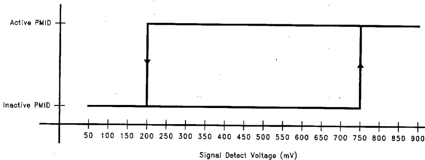
FIGURE 17. Signal Detect
