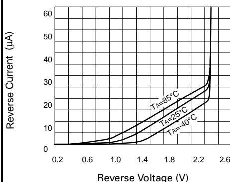
Reverse Characteristics
