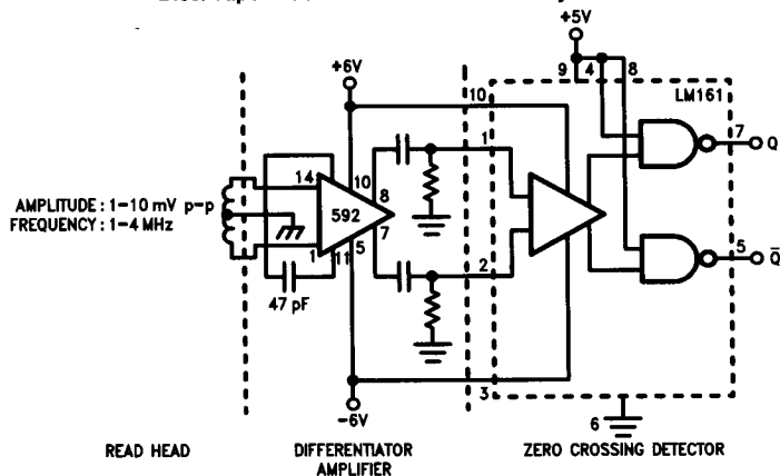
Disc/Tape Phase Modulated Readback Systems
