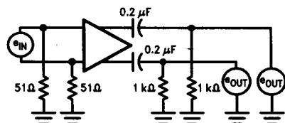
Test Circuit 2
