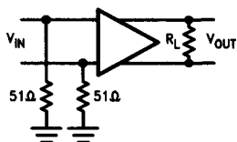
Test Circuit 1
