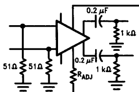
Voltage Gain Adjust Circuit
