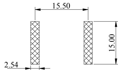
( PCB Pattern )
