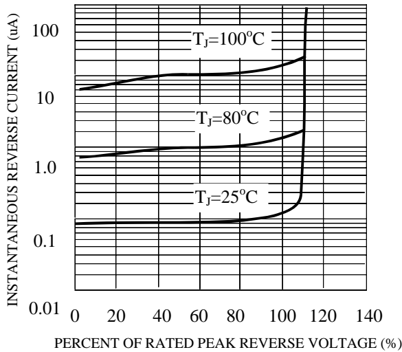
FIG. 3-TYPICAL REVERSE CHARACTERISTICS
