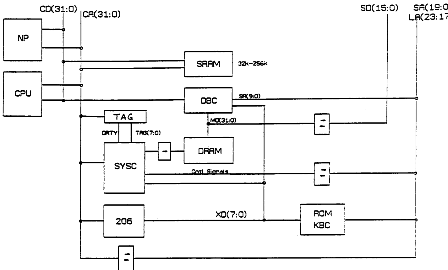
BLOCK DIAGRAM
