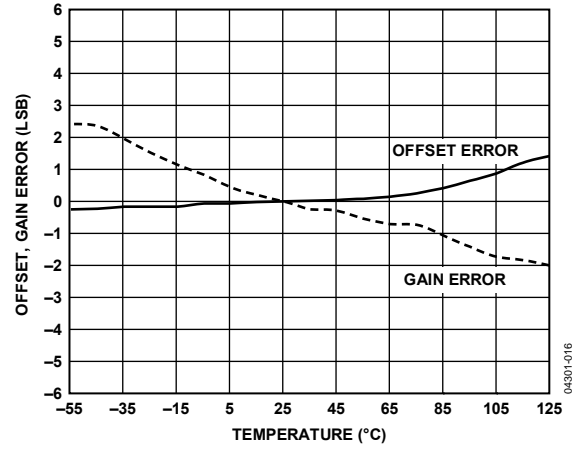
Figure 19. Offset and Gain Error vs. Temperature
