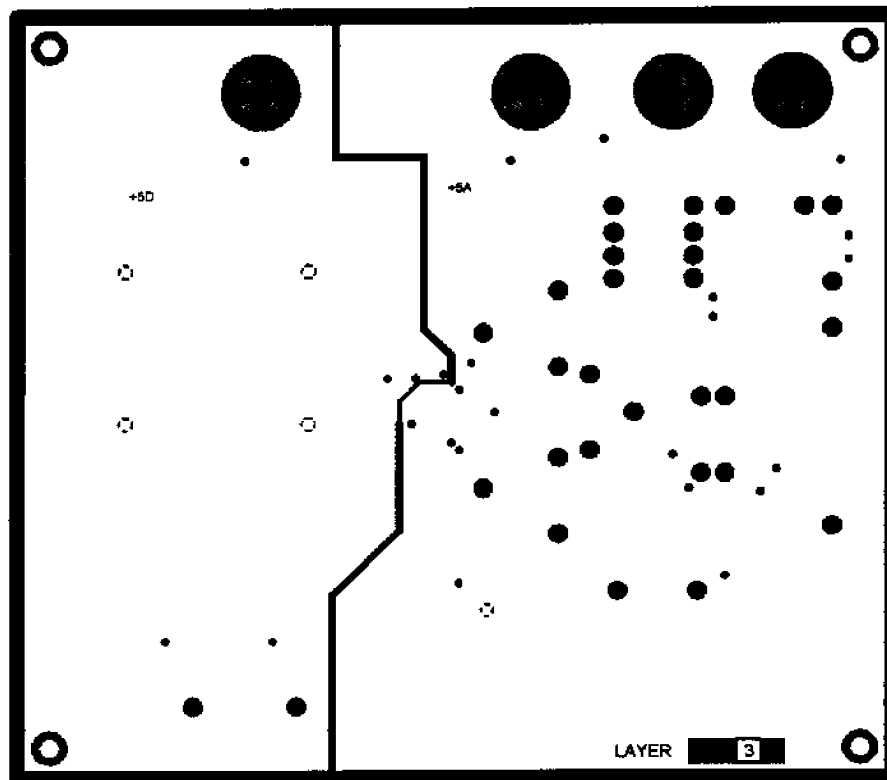
Figure 63. Power Plane PCB Layout (Layer 3)
