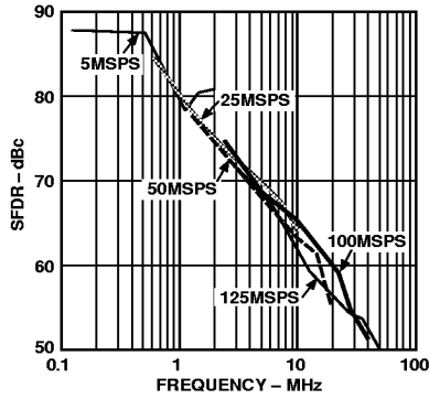
Figure 3. SFDR vs. f_{OUT} @ 0 dBFS
