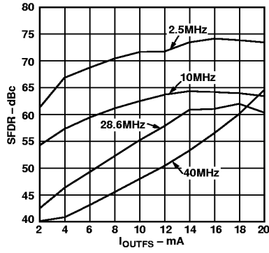
Figure 13. SFDR vs. f_{\text{OUT}} and I_{\text{OUTFS}} @ 100 MSPS, 0 dBFS
