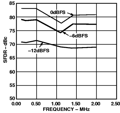
Figure 4. SFDR vs. f_{OUT} @ 5 MSPS
