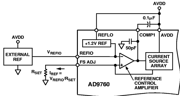
Figure 41. External Reference Configuration
