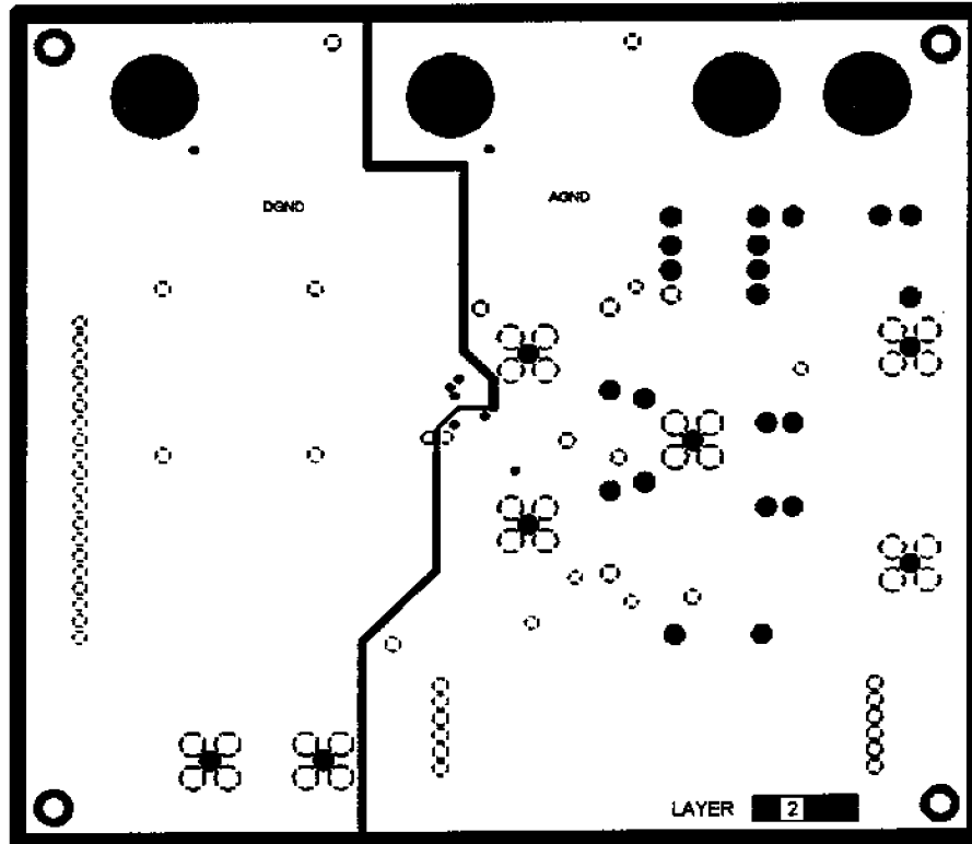
Figure 62. Ground Plane PCB Layout (Layer 2)
