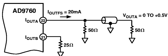
Figure 53. 0 V to +0.5 V Unbuffered Voltage Output
