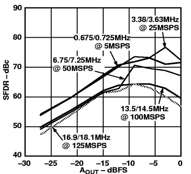
Figure 29. Dual-Tone SFDR vs. A_{OUT} @ f_{OUT} = f_{CLOCK}/7
