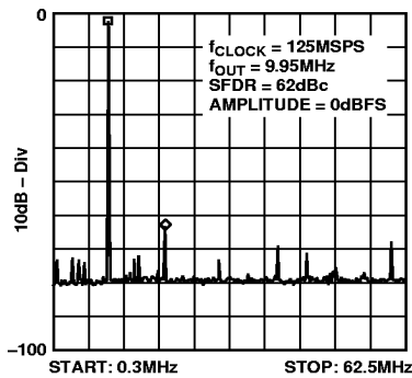
Figure 18. Single-Tone SFDR
