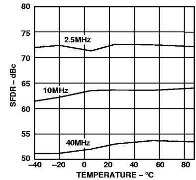
Figure 17. SFDR vs. Temperature @ 100 MSPS, 0 dBFS
