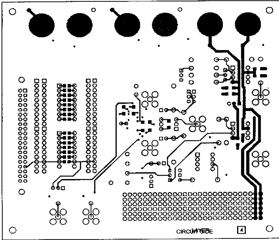
Figure 64. Solder Side PCB Layout (Layer 4)
