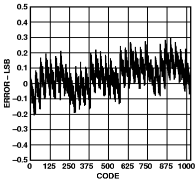
Figure 15. Typical INL
