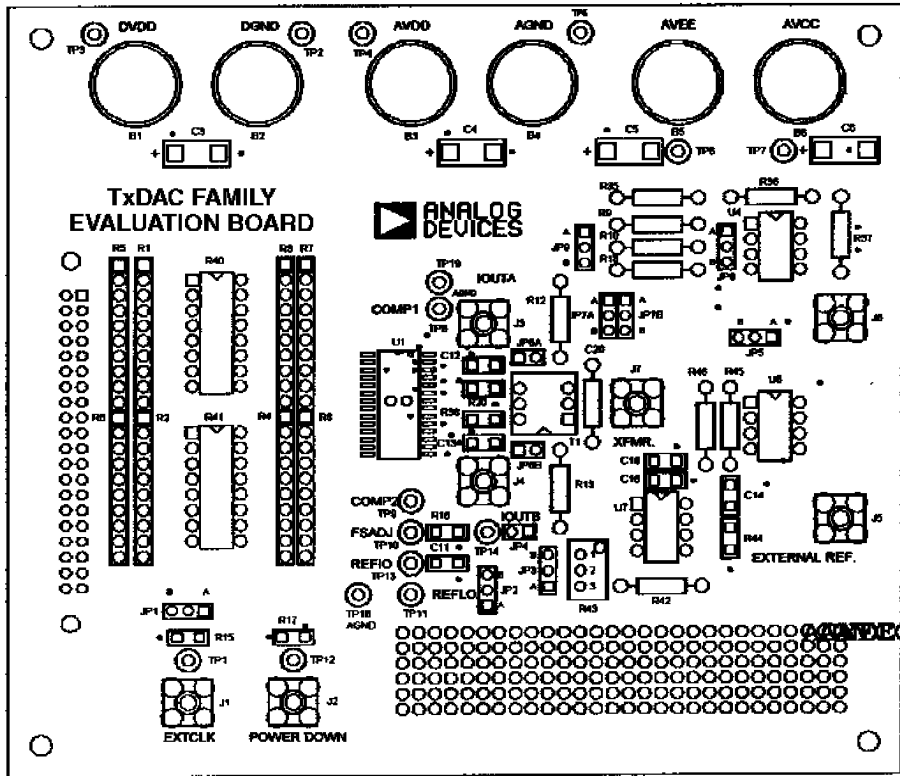
Figure 60. Silkscreen Layer—Top
