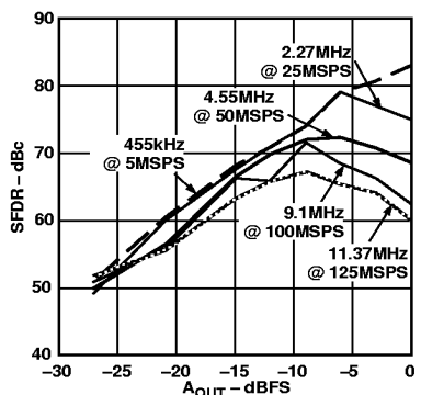
Figure 27. Single-Tone SFDR vs. A_{OUT} @ f_{OUT} = f_{CLOCK}/11
