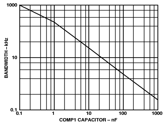
Figure 42. External COMP1 Capacitor vs. -3 dB Bandwidth
