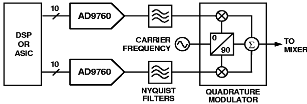
Figure 56. Typical Analog QAM Architecture
