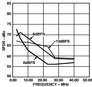
Figure 25. SFDR vs. f_{OUT} @ 100 MSPS
