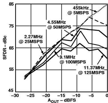
Figure 9. Single-Tone SFDR vs. A_{OUT} @ f_{OUT} = f_{CLOCK}/11
