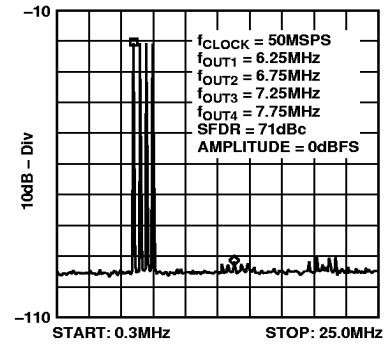
Figure 38. Four-Tone SFDR
