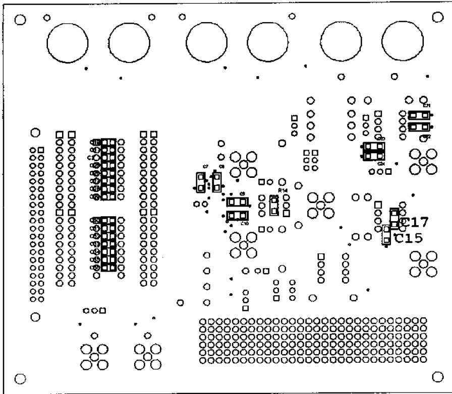
Figure 65. Silkscreen Layer—Bottom
