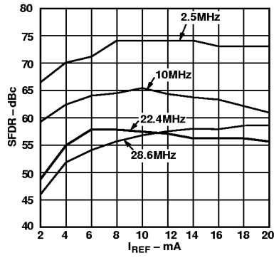
Figure 31. SFDR vs. f_{\text{OUT}} and I_{\text{OUTFS}} @ 100 MSPS, 0 dBFS
