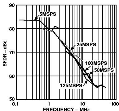
Figure 21. SFDR vs. f_{OUT} @ 0 dBFS
