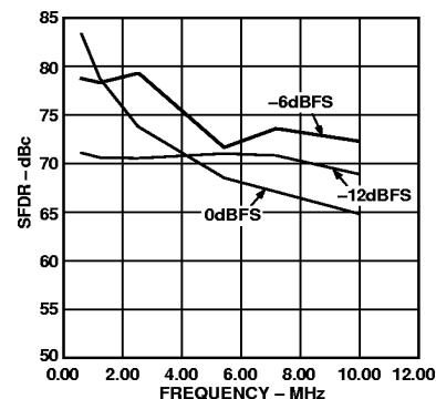
Figure 23. SFDR vs. f_{OUT} @ 25 MSPS
