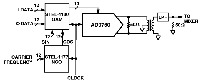
Figure 58. Digital QAM Architecture
