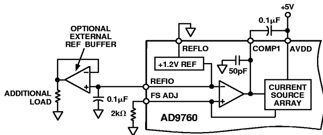
Figure 40. Internal Reference Configuration
