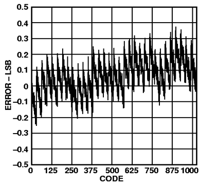
Figure 33. Typical INL
