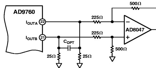
Figure 51. DC Differential Coupling Using an Op Amp
