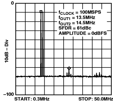
Figure 19. Dual-Tone SFDR
