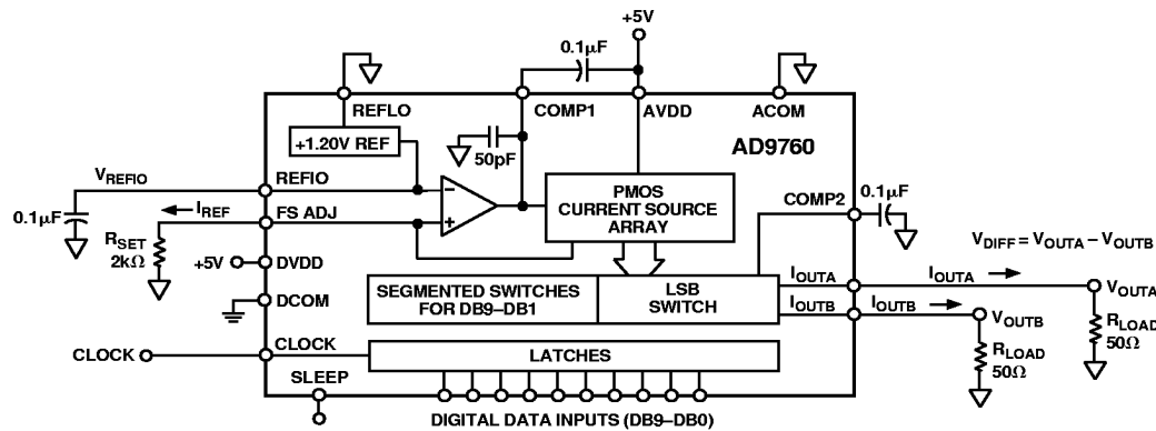
Figure 39. Functional Block Diagram
