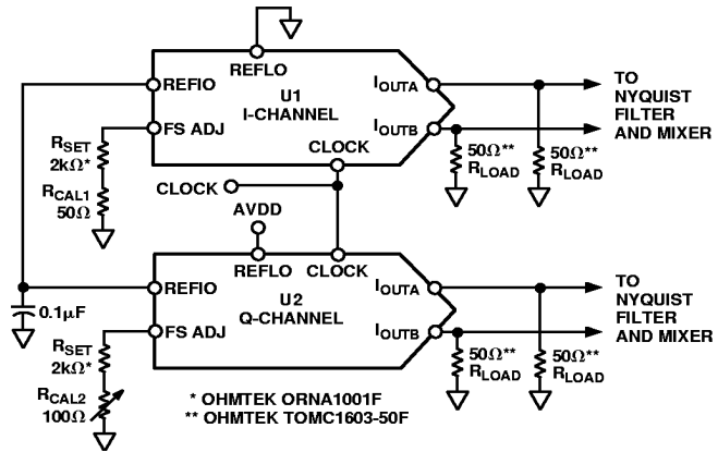
Figure 57. Baseband QAM Implementation Using Two AD9760s
