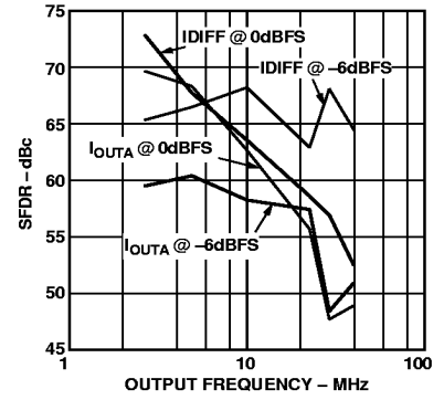
Figure 14. Differential vs. Single-Ended SFDR vs. f_{\text{OUT}} @ 100 MSPS
