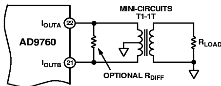
Figure 50. Differential Output Using a Transformer
