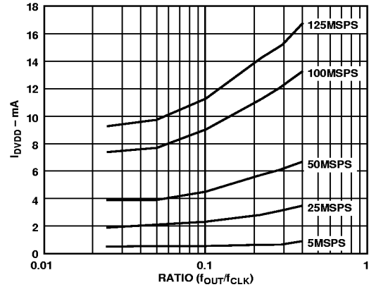
Figure 48. I DVDD vs. Ratio @ DVDD = 5 V
