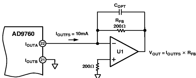
Figure 54. Unipolar Buffered Voltage Output
