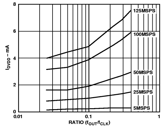
Figure 49. I DVDD vs. Ratio @ DVDD = 3 V
