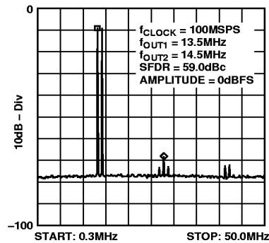
Figure 37. Dual-Tone SFDR
