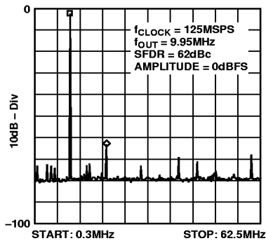
Figure 36. Single-Tone SFDR
