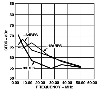
Figure 26. SFDR vs. f_{OUT} @ 125 MSPS
