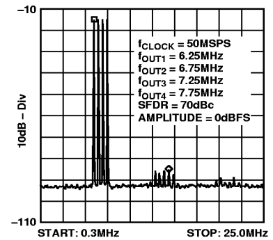
Figure 20. Four-Tone SFDR
