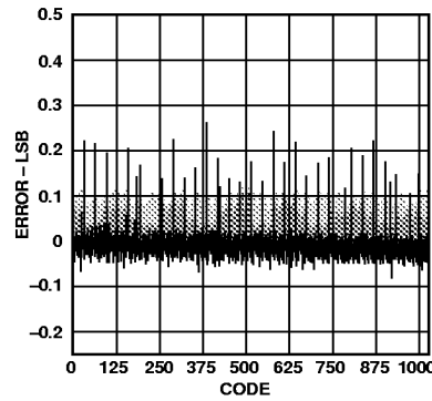
Figure 16. Typical DNL
