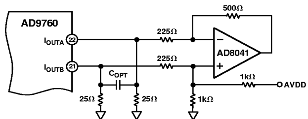
Figure 52. Single-Supply DC Differential Coupled Circuit
