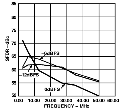
Figure 8. SFDR vs. f_{OUT} @ 125 MSPS
