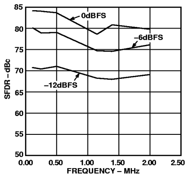
Figure 22. SFDR vs. f_{OUT} @ 5 MSPS
