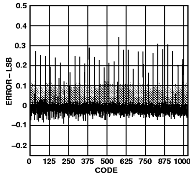
Figure 34. Typical DNL
