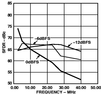
Figure 7. SFDR vs. f_{OUT} @ 100 MSPS
