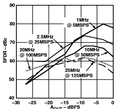
Figure 28. Single-Tone SFDR vs. A_{OUT} @ f_{OUT} = f_{CLOCK}/5
