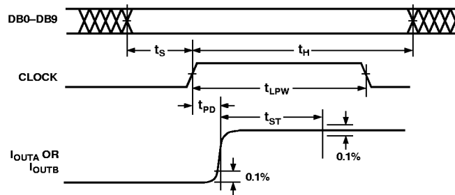
Figure 1. Timing Diagram
