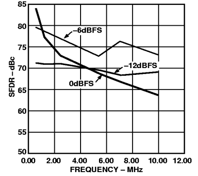
Figure 5. SFDR vs. f_{OUT} @ 25 MSPS
