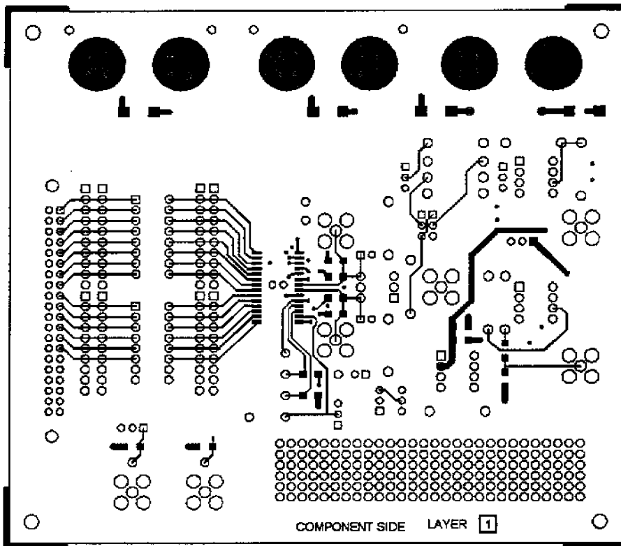
Figure 61. Component Side PCB Layout (Layer 1)
