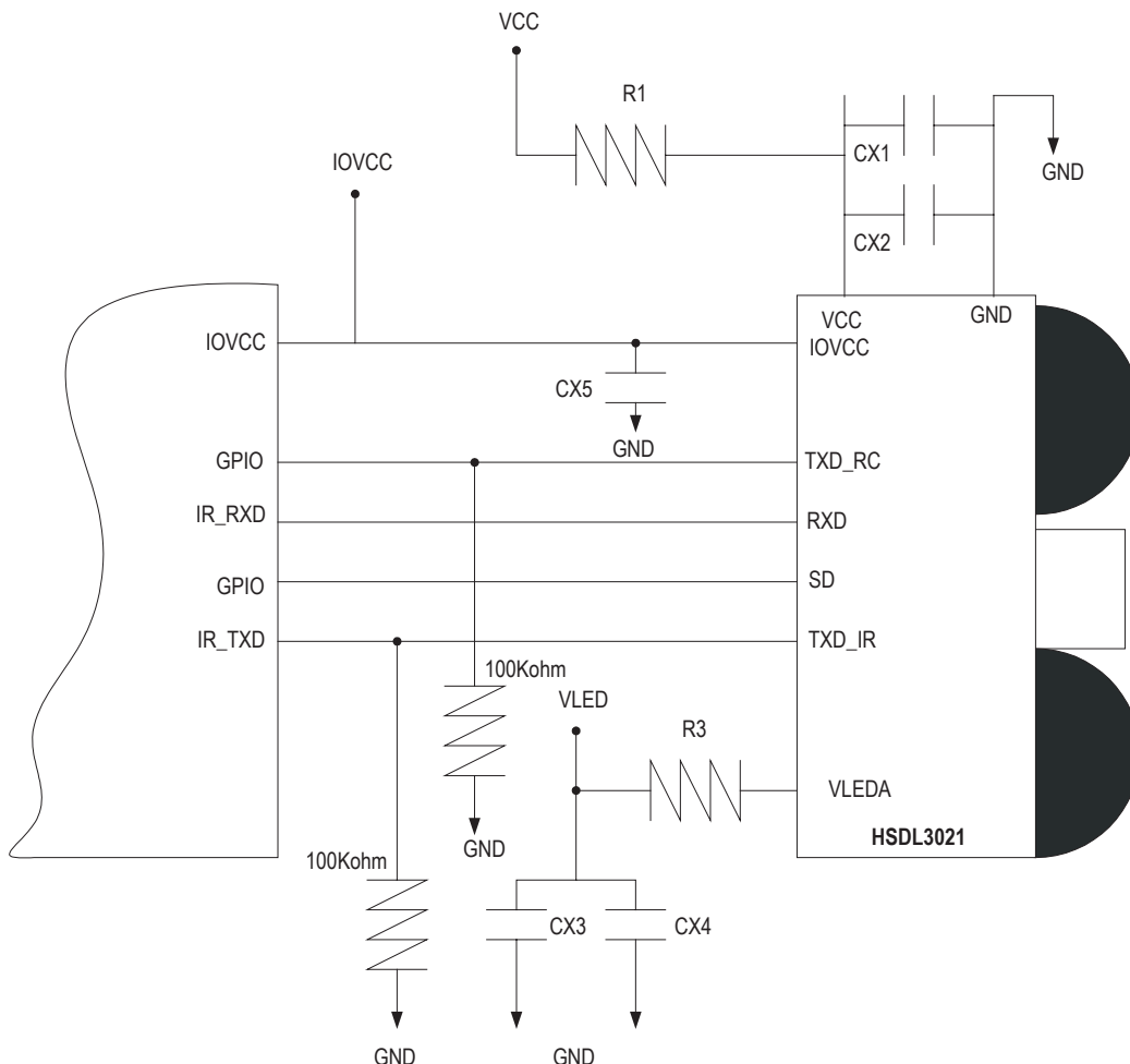
Figure 3. ASDL-3023 configuration with general mobile architecture processor
