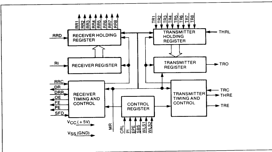
TR1863/TR1865 BLOCK DIAGRAM
