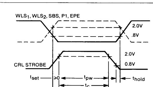
FIGURE 3. CONTROL REGISTER LOAD CYCLE
