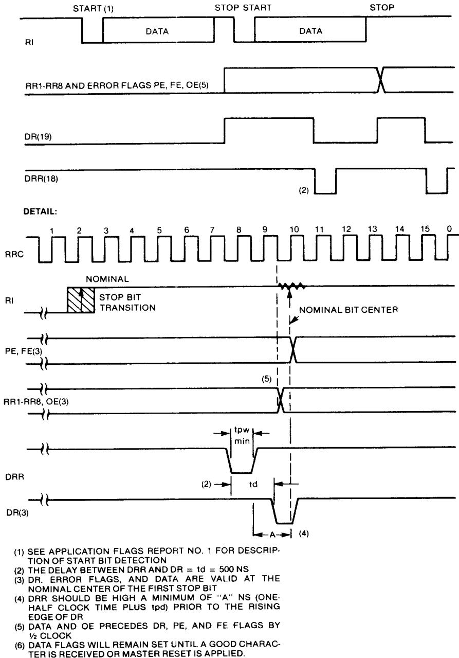
FIGURE 1. RECEIVER TIMING
