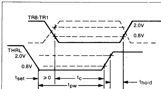
FIGURE 2. DATA INPUT LOAD CYCLE
