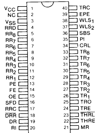
PIN DESIGNATION
