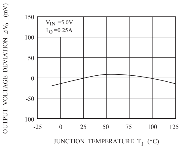
Fig.5-3 T_j - \Delta V_O (KIA78MR33)
