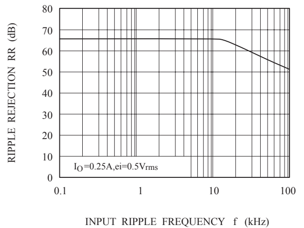
Fig.8 f - \text{RR}
