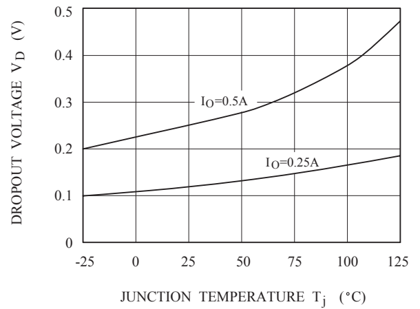
Fig.6 T_j - V_D
