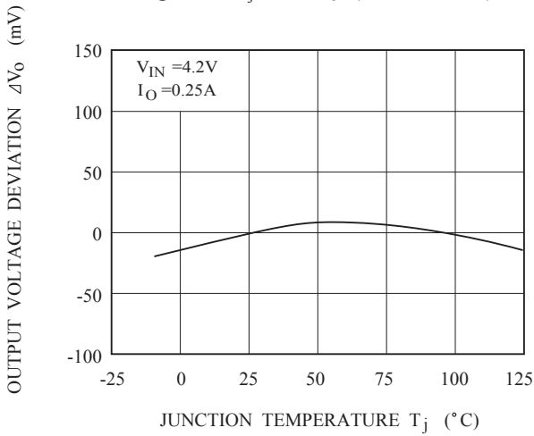
Fig.5-1 T_j - \Delta V_O (KIA78MR25)
