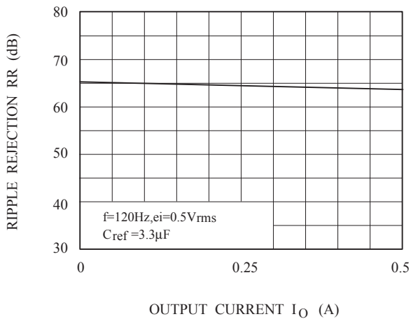
Fig.9 I_O - \text{RR}
