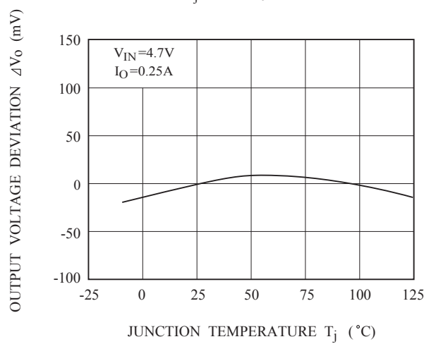
Fig.5-2 T_j - \Delta V_O (KIA78MR30)
