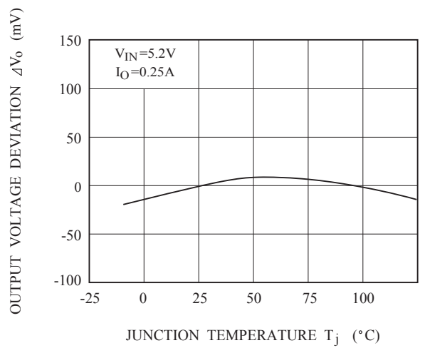
Fig.5-4 T_j - \Delta V_O (KIA78MR35)
