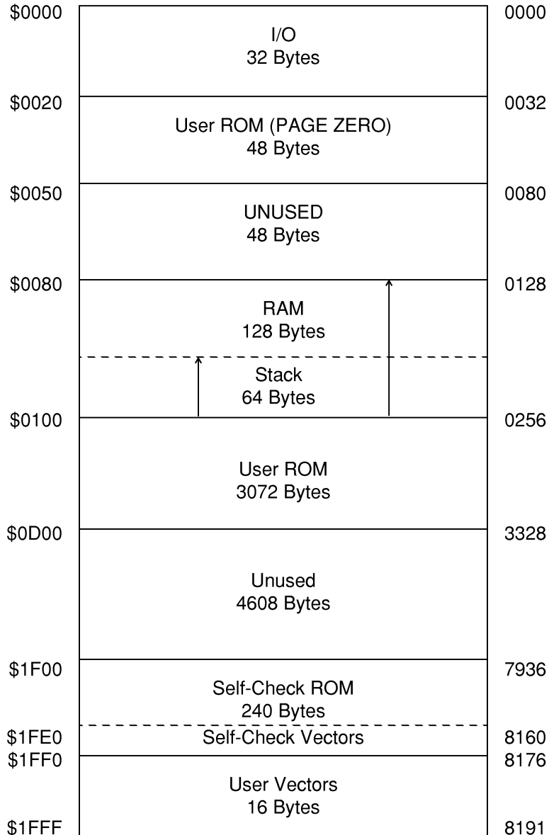
Figure 3-1: The 8K Memory Map of the MC68HC05P5
