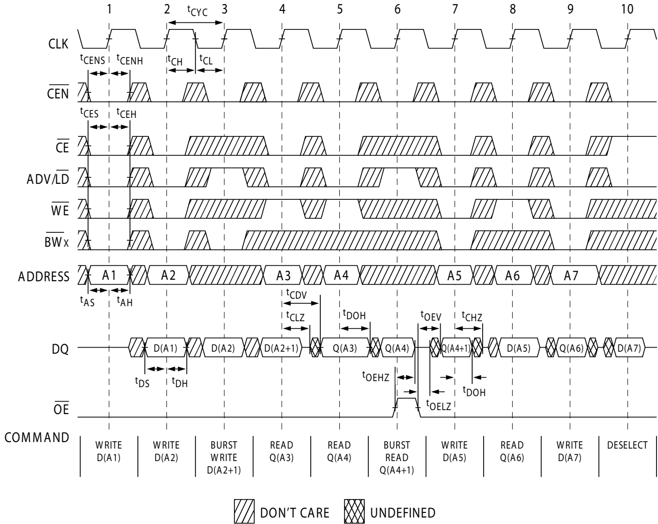
Figure 2. Read/Write Waveforms [26, 27, 28]
