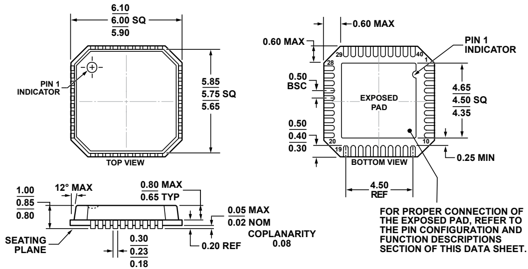
Figure 55. 40-Lead Lead Frame Chip Scale Package [LFCSP_VQ] 6 mm × 6 mm Body, Very Thin Quad (CP-40-13) Dimensions shown in millimeters
