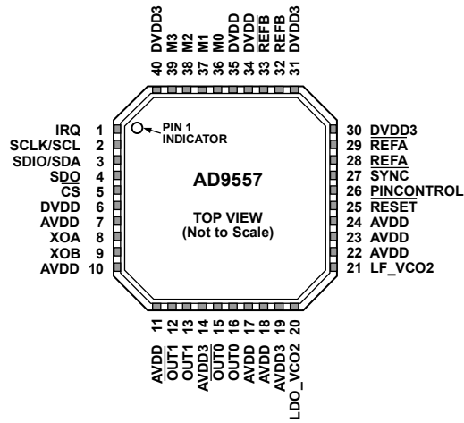
Figure 2. Pin Configuration
