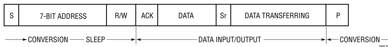
Figure 6. Conversion Sequence
