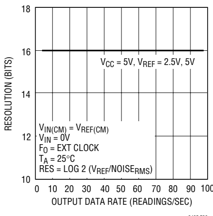
Figure 36. Resolution ( Noise_{RMS} \le 1LSB ) vs Output Data Rate and Temperature
