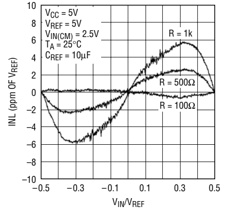
Figure 17. INL vs Differential Input Voltage and Reference Source Resistance for C REF > 1μF
