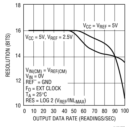
Figure 37. Resolution ( INL_{MAX} \le 1LSB ) vs Output Data Rate and Temperature
