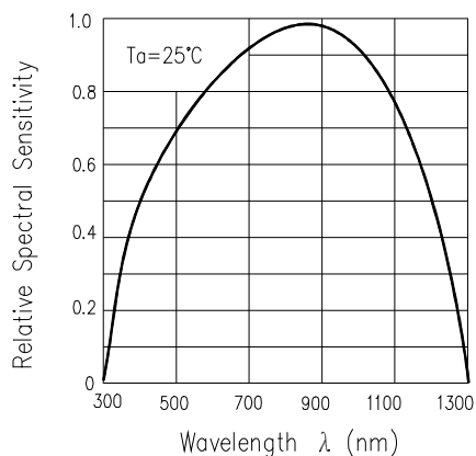
Fig.5 Spectral Sensitivity
