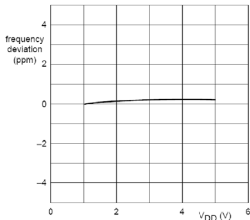
T amb = 25 °C; normalized to V DD = 3 V. Frequency deviation as function of V DD .
