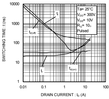
Fig.14 Switching Characteristics
