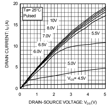
Fig. 3 Typical output characteristics(11)
