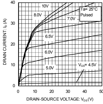
Fig. 2 Typical output characteristics(1)
