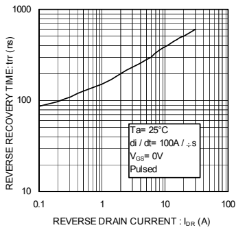
Fig.13 Reverse Recovery Time vs. Reverse Drain Current
