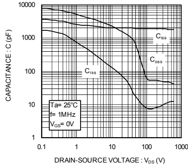
Fig.11 Typical Capacitance vs. Drain-Source Voltage
