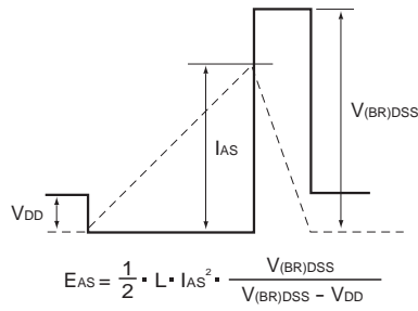
Fig.3-2 Avalanche waveform
