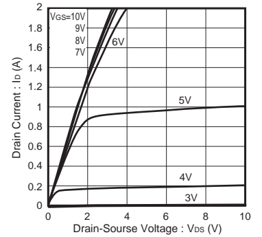
Fig.12 Typical Output Characteristics
