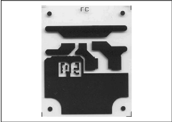
Figure 10. PCB layout (front side)
