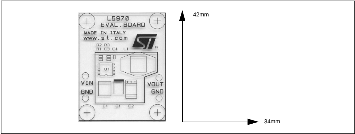
Figure 8. PCB layout (component side)
