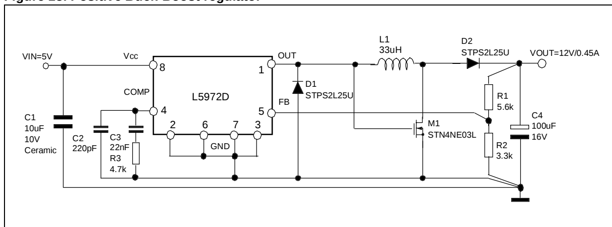
Figure 14. Buck-Boost regulator
