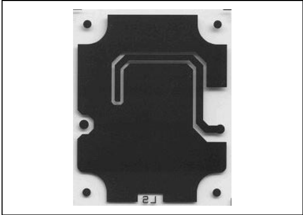
Figure 9. PCB layout (bottom side)
