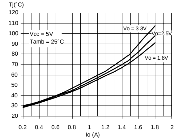
Figure 12. Junction Temperature vs. Output Current
