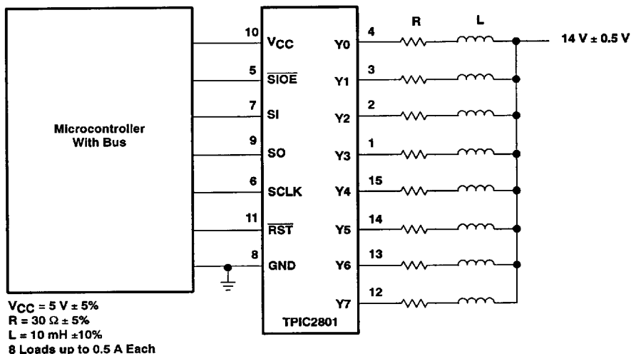
Figure 6. Microcontroller Driving Eight Loads Using a TPIC2801 for Load Interface
