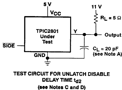
Figure 3. Test Circuit and Voltage Waveforms for Delay Times
