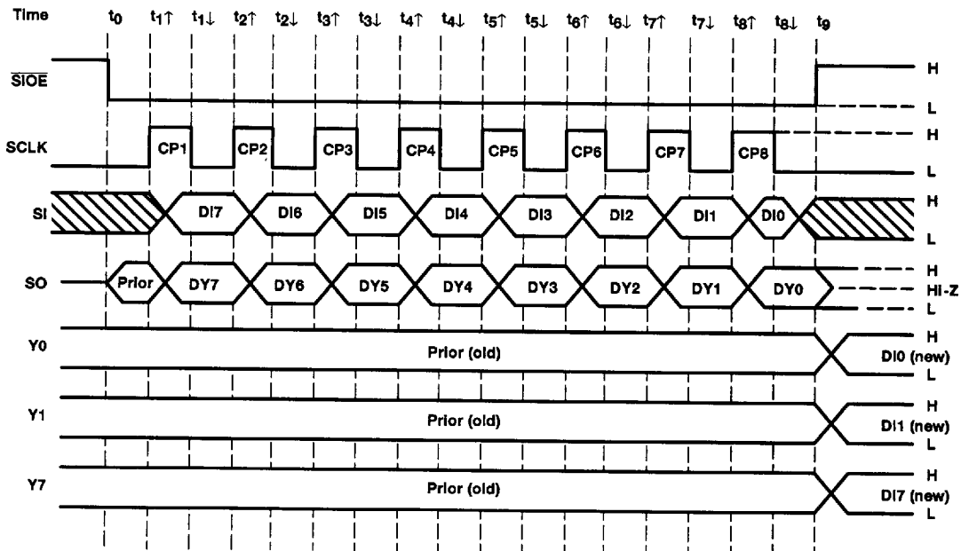
Figure 7. Data-Byte Transfer Timing
