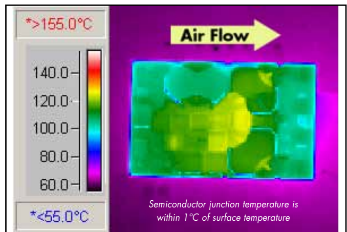
Figure 6: Thermal plot of converter at 11.2 amp load current (134W) with 55°C air flowing at the rate of 200 LFM. Air is flowing across the converter from input to output (nominal input voltage).
