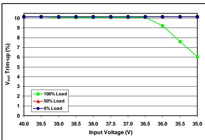
Figure 23: Percentage of output voltage trim-up that can be achieved at various input voltages from 35V-40V and output loads of 0%, 50% and full load.
