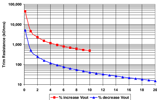
Figure C: Trim Graph for 12.0Vout module
