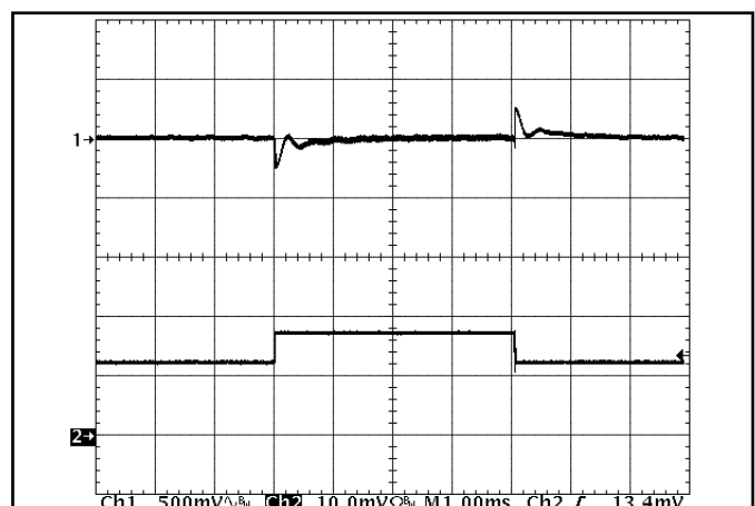
Figure 12: Output voltage response to step-change in load current (50%-75%-50% of I_{out(max)} ; dI/dt = 1\text{A}/\mu\text{s} ). Load cap: 470 \mu\text{F} , 30 m \Omega ESR tantalum capacitor and 1 \mu\text{F} ceramic cap. Ch 1: V_{out} (500mV/div), Ch 2: I_{out} (5A/div).
