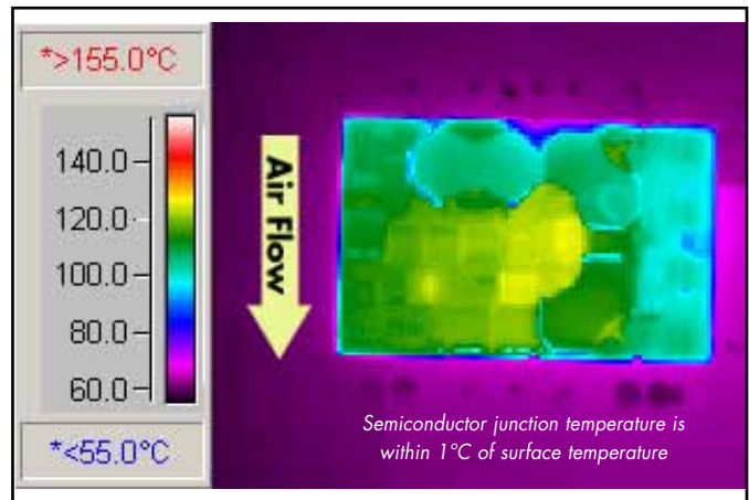
Figure 8: Thermal plot of converter at 11.6 amp load current (139W) with 55°C air flowing at the rate of 200 LFM. Air is flowing from pin 1 to pin 3 (nominal input voltage).
