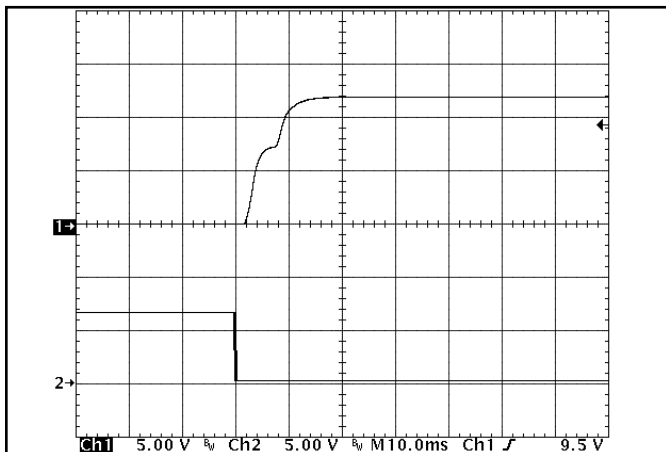
Figure 9: Turn-on transient at full rated load (resistive load) (10 ms/div) Input voltage pre-applied. Ch 1: V_{out} (5V/div). Ch 2: ON/OFF input (5V/div)
