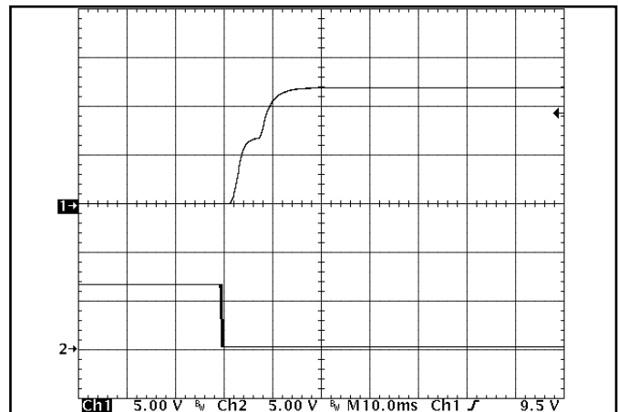
Figure 10: Turn-on transient at zero load current (10 ms/div). Ch 1: V_{out} (5V/div). Ch 2: ON/OFF input (5V/div)
