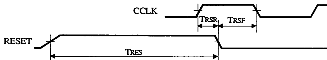
RESET Timing
