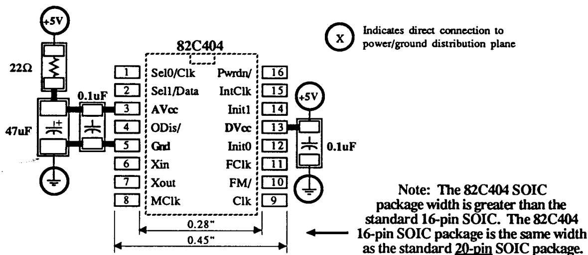
82C404 Recommended PCB Layout
