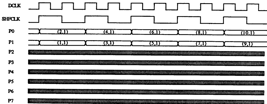
Monochrome, Single Drive, 2 pixels/clock, CD = 01, FRC = 00, 01, 10
