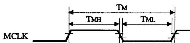
Clock Timing
