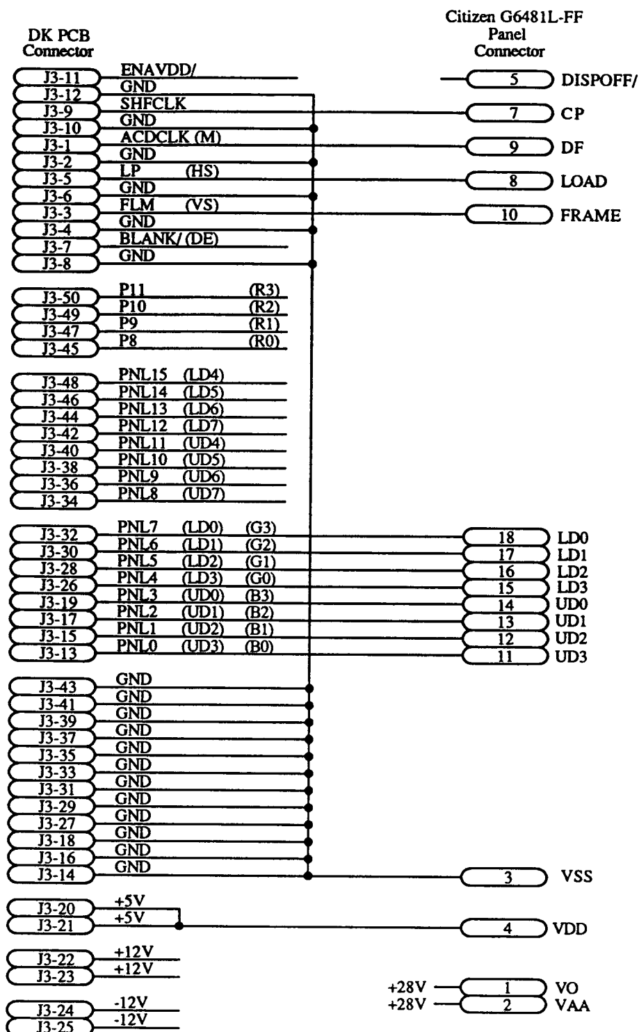
65520 / 530 Interface - Citizen G6481L-FF (640x480 Monochrome LCD DD Panel)
