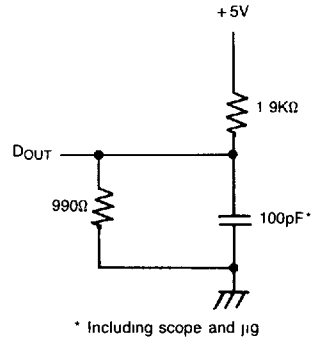
Fig. 1 Output Load Circuit
