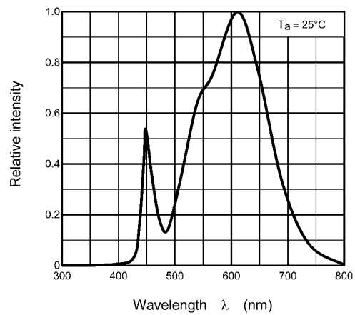
Fig. 8.4 Wavelength characteristic
