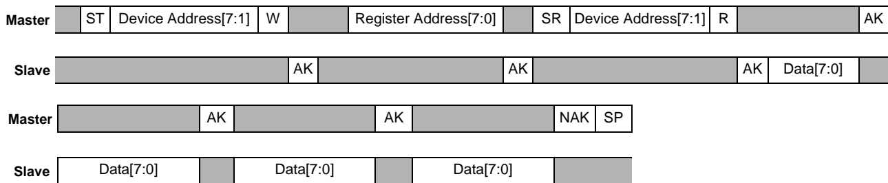
Figure 12. Multiple Byte Read timing (I 2 C)
