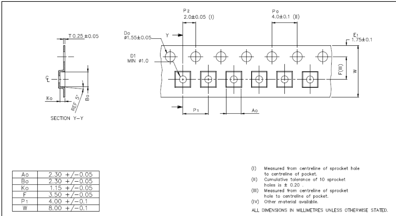
Figure 63. Carrier tape
