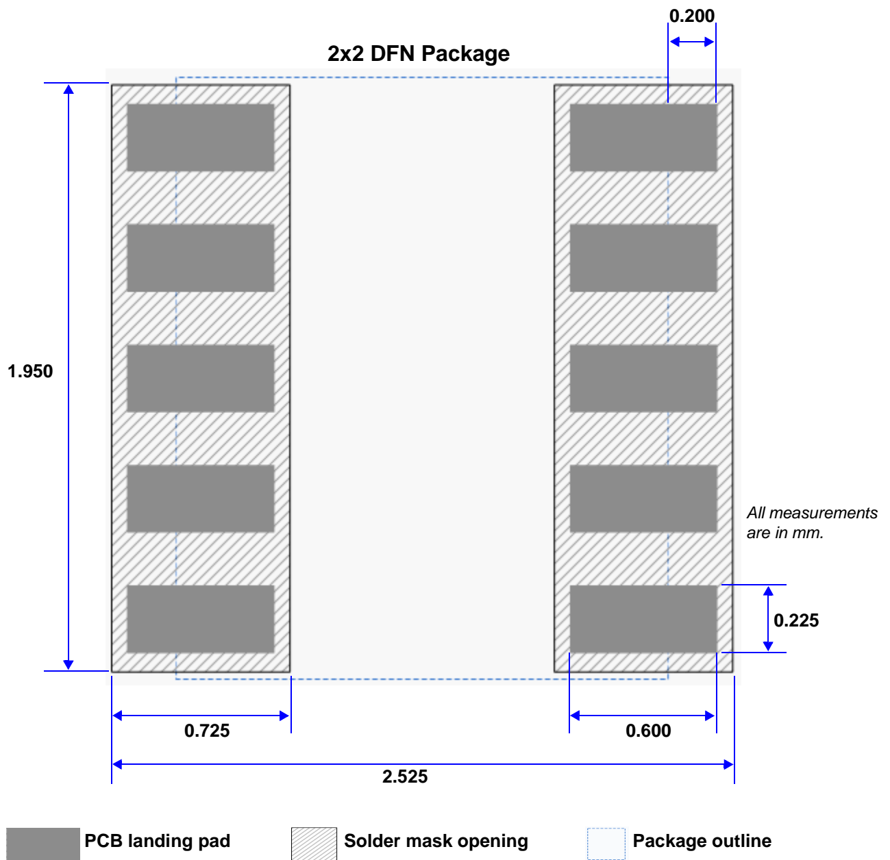
Figure 62. Package mounting measurements
