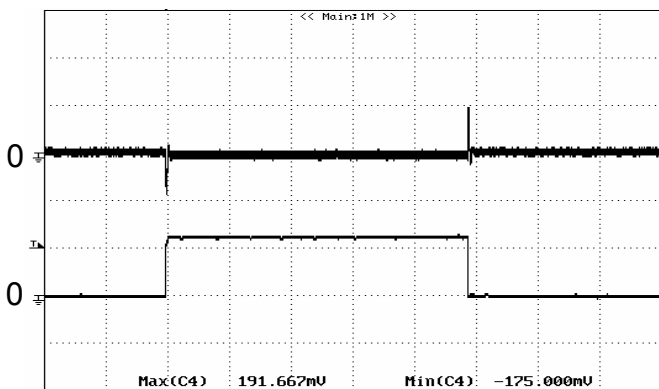
Figure 17: Typical transient response to step load change at 10A/μS from 50%~100% load, at 12Vin, 2.5V out
