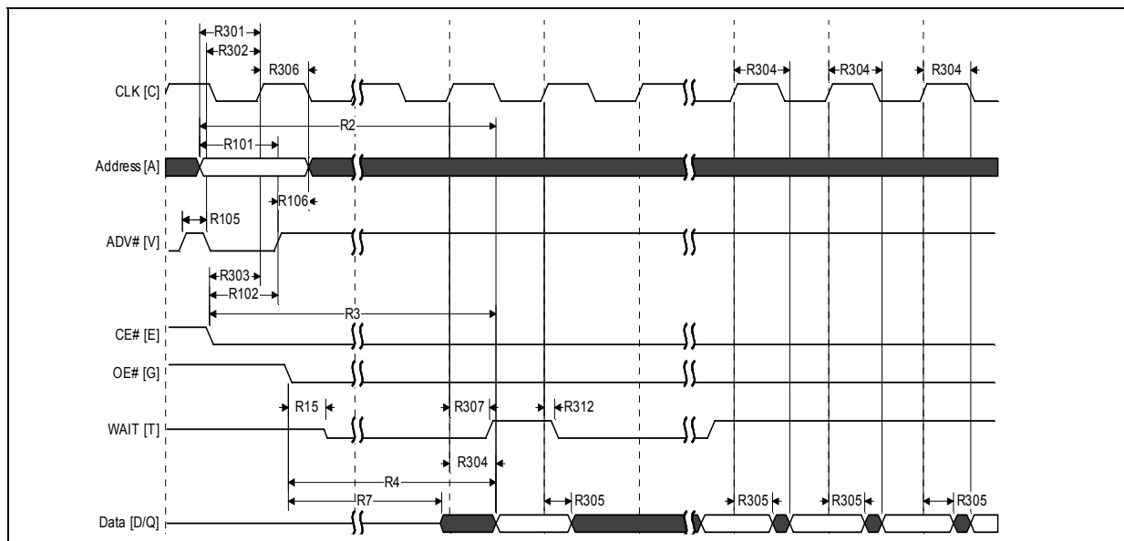
Figure 15: Continuous Burst Read, showing an Output Delay Timing
