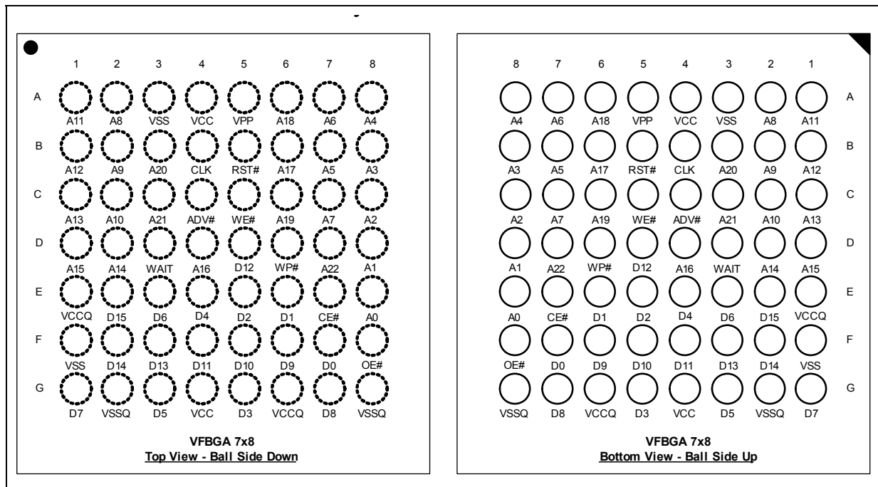
Figure 5: 7x8 Active-Ball Matrix for 128-Mbit Density in VF BGA Packages
