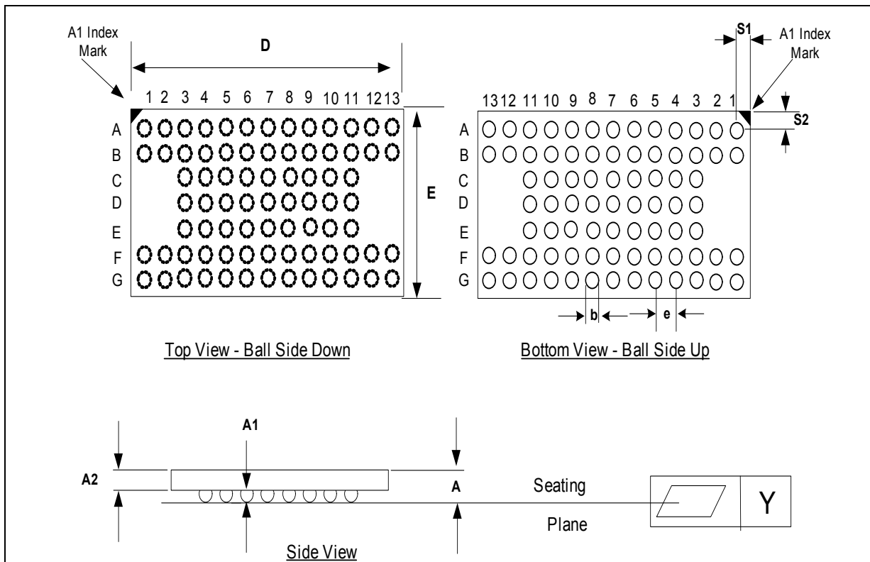
Figure 2: 256-Mbit, 79-Ball VF BGA Package Drawing and Dimensions
