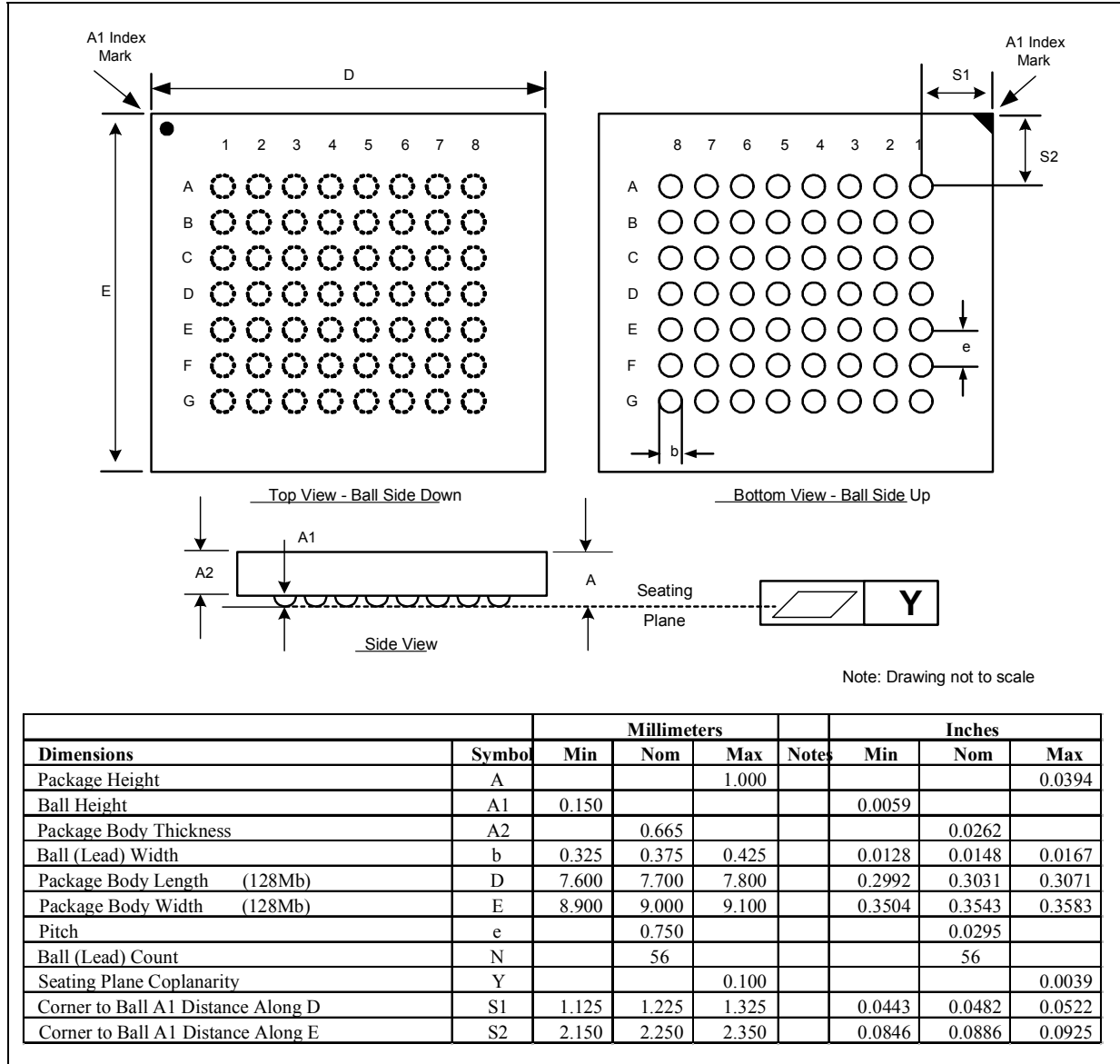
Figure 1: 128-Mbit, 56-Ball VF BGA Package Drawing and Dimensions
