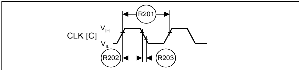
Figure 10: Clock Input AC Waveform
