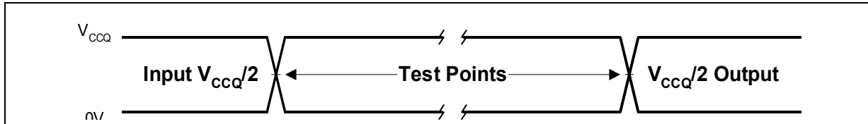
Figure 8: AC Input/Output Reference Waveform
