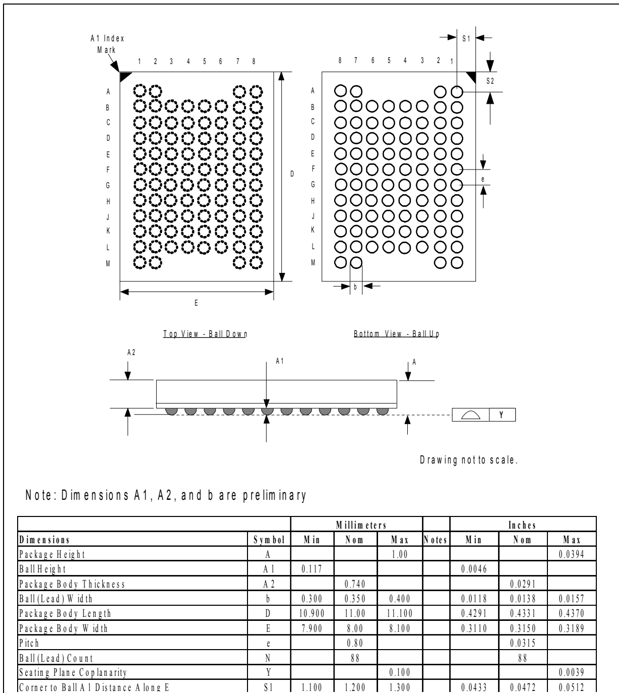
Figure 4: 256-Mbit, 88-ball (80-active ball) Drawing and Dimensions (8x11x1.0 mm)
