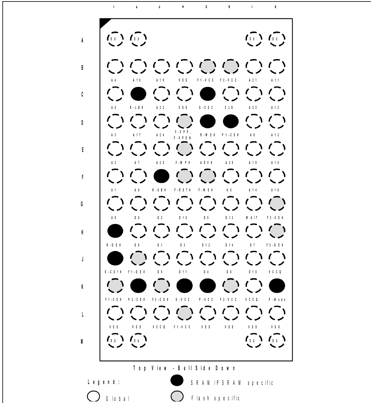
Figure 7: 88-Ball (80-Active Ball) SCSP Package Ballout
