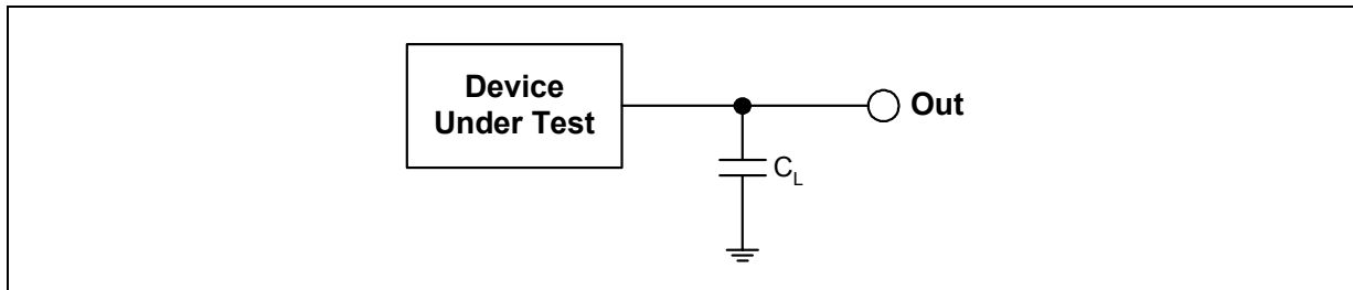
Figure 9: Transient Equivalent Testing Load Circuit
