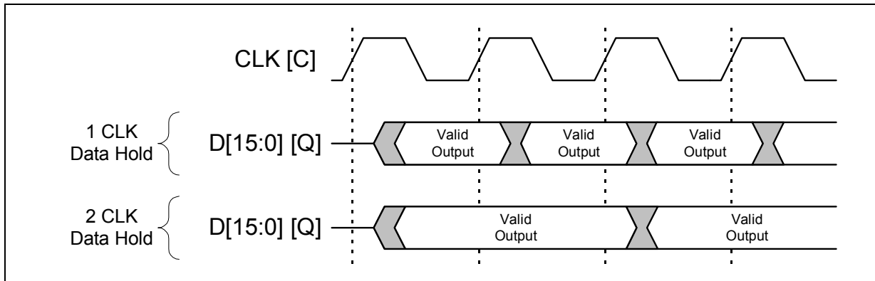
Figure 26: Data Hold Timing
