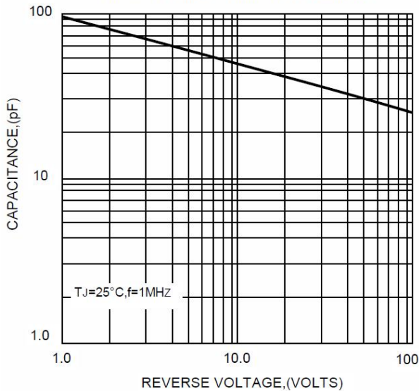
FIG.3-TYPICAL JUNCTION CAPACITANCE
