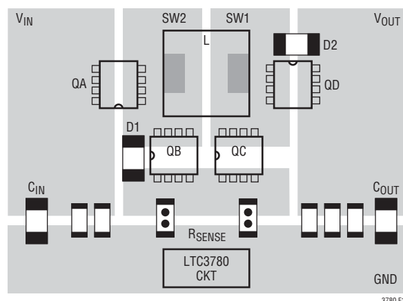
Figure 10. Switches Layout
