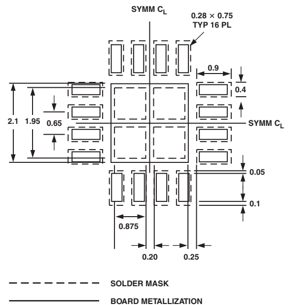
Figure 2. 16-Lead 4 x 4 Land Pattern
