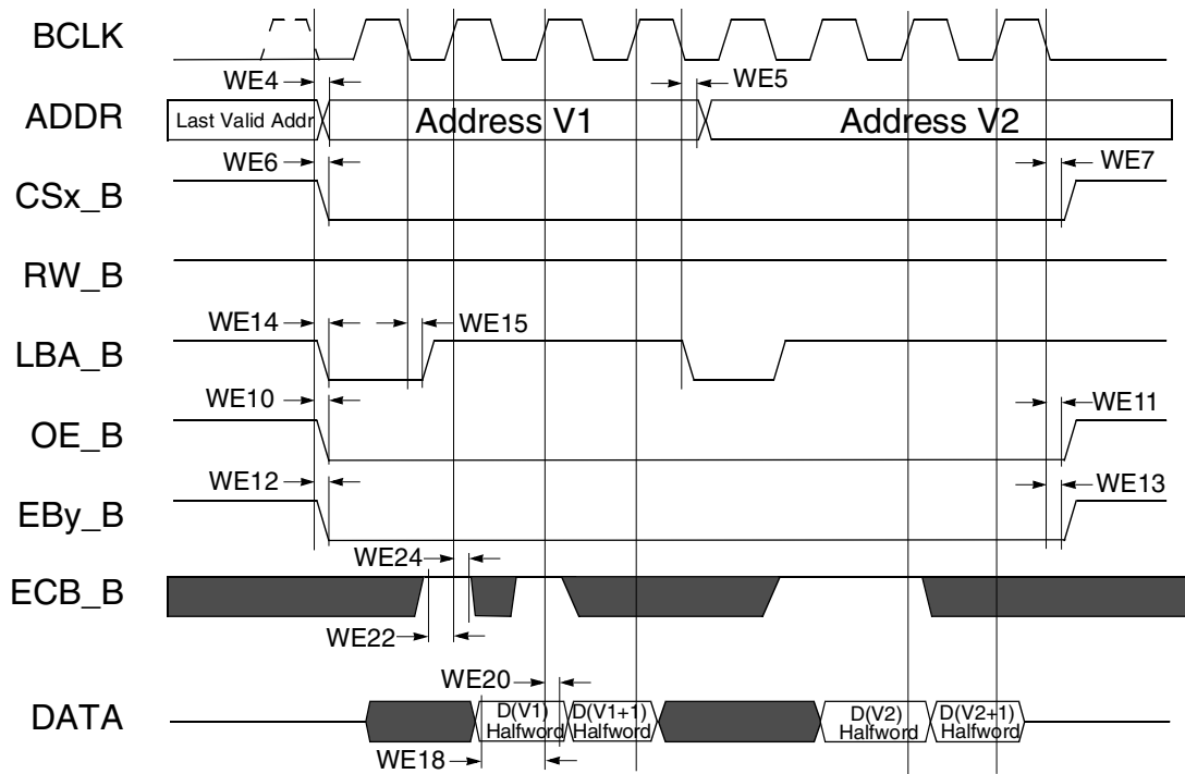
Figure 16. Synchronous 16-Bit Memory, Two Non-Sequential 32-Bit Read Accesses, WSC=2, SYNC=1, DOL=0
