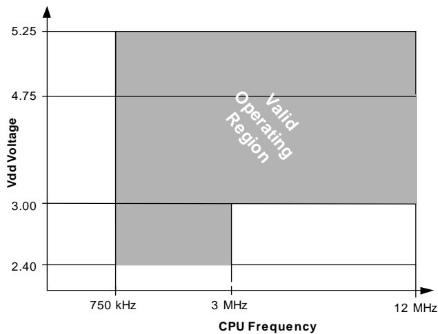
Figure 2-1a. Voltage versus CPU Frequency
