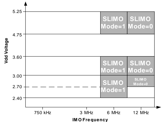
Figure 2-1b. IMO Frequency Trim Options
