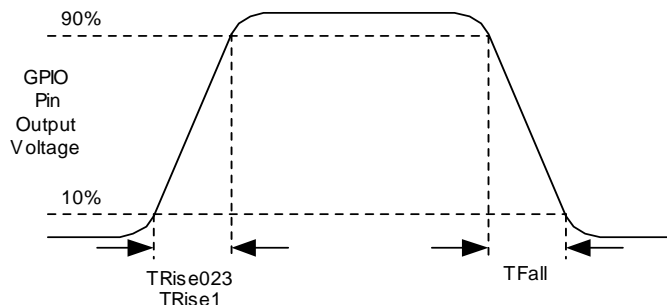
Figure 2-2. GPIO Timing Diagram
