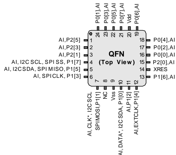
CY8C20334 24-Pin PSoC Device
