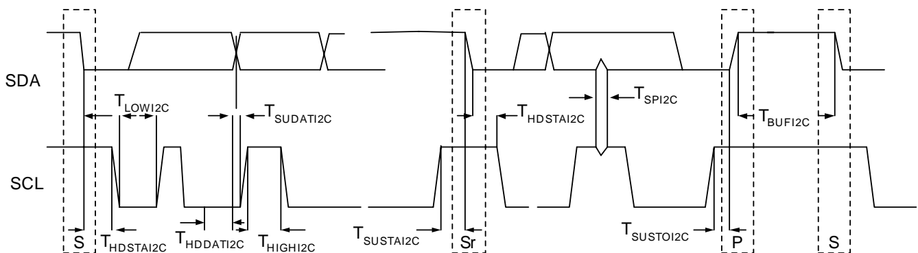
Figure 2-3. Definition for Timing for Fast/Standard Mode on the I 2 C Bus
