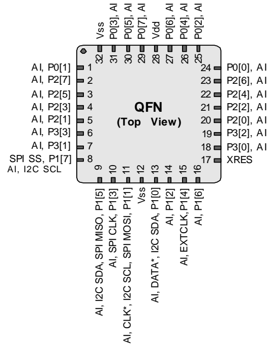
CY8C20434 32-Pin PSoC Device
