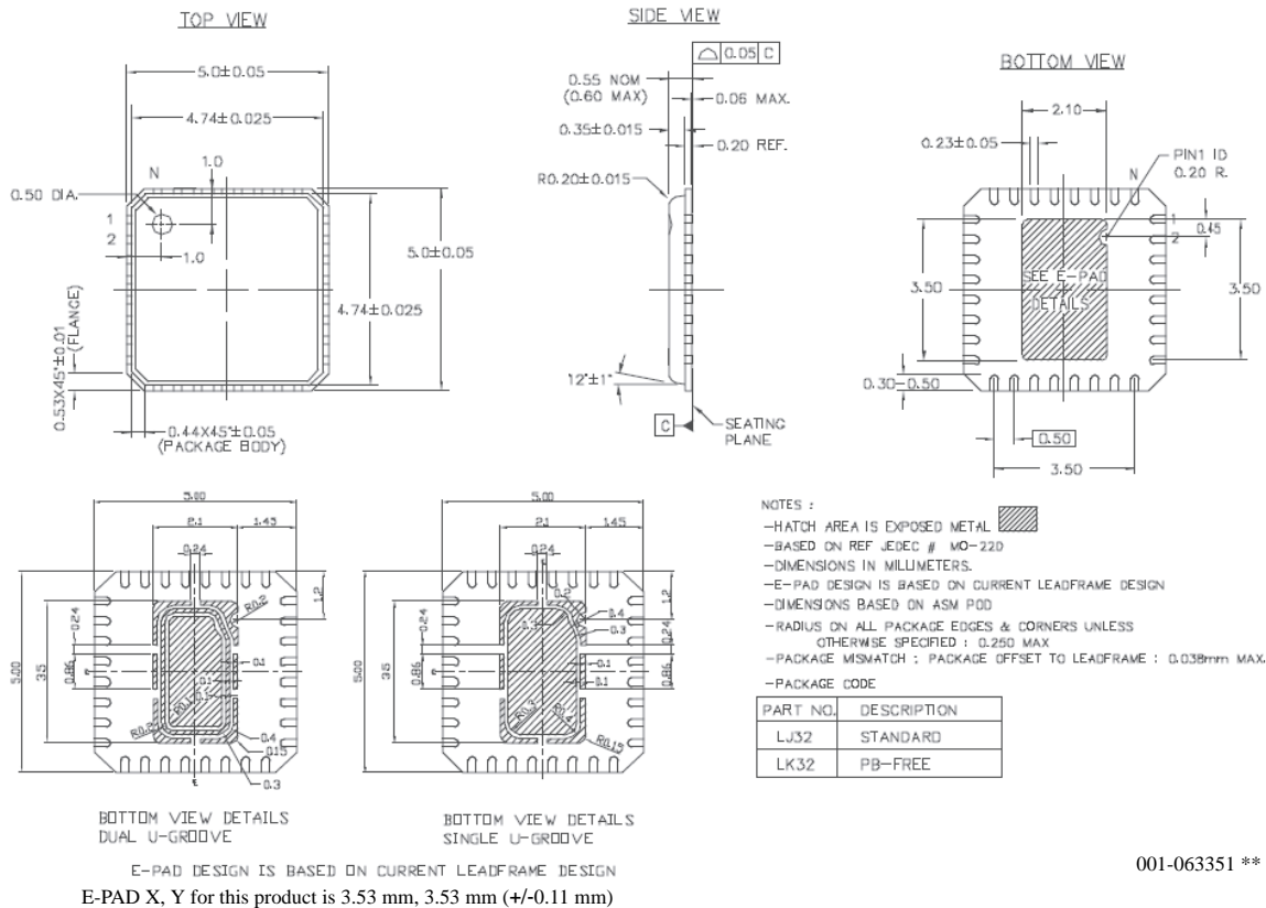
Figure 3-2. 32-Lead (5x5 mm) QFN
