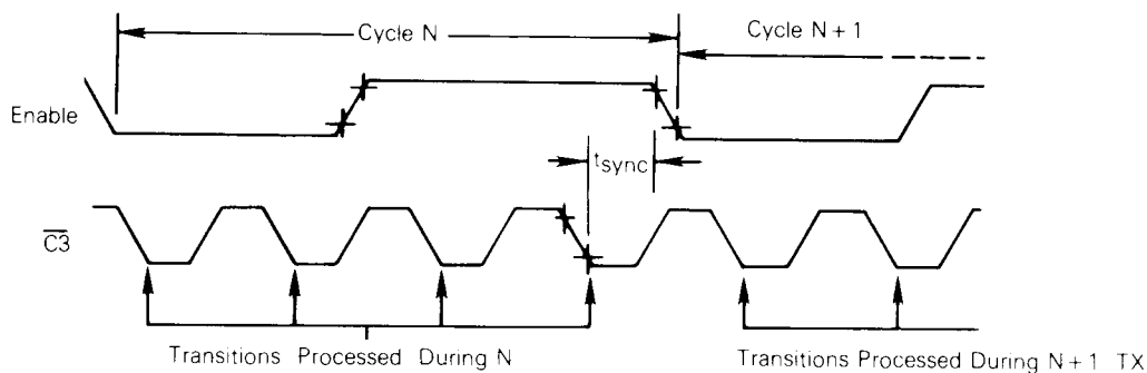
FIGURE 7 — \overline{C3} INPUT SYNCHRONIZATION TIME ( \pm 8 PRESCALER MODE ONLY)
