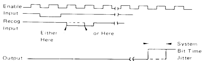
FIGURE 9 — INPUT JITTER
