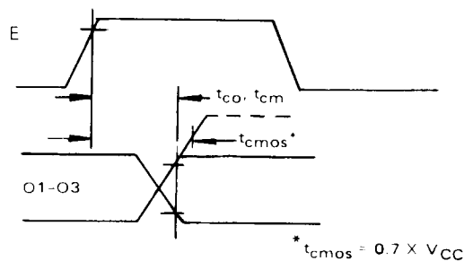
FIGURE 5 — OUTPUT DELAY
