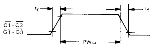
FIGURE 3 — INPUT PULSE WIDTH HIGH
