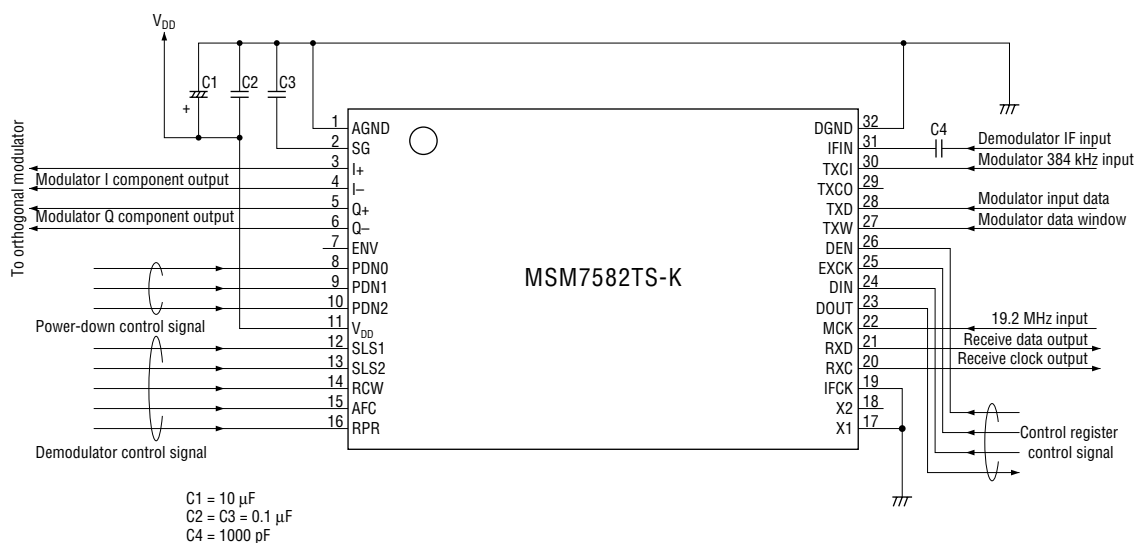
Figure 11 Example of Circuit Configuration
