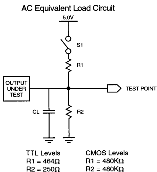
Figure 12: PEEL18CV8 AC Test Loads/Waveforms
