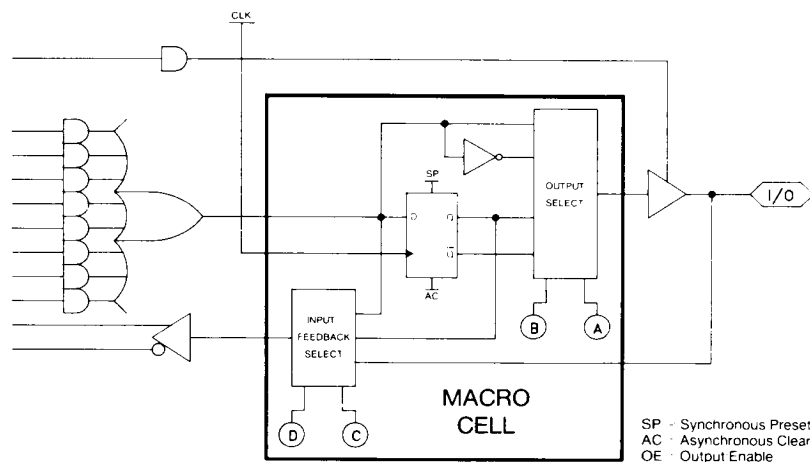
Figure 9: PEEL18CV8 Macrocell Diagram
