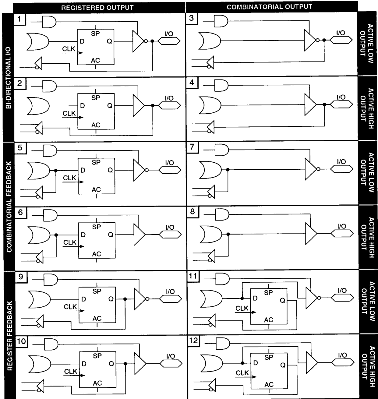
Figure 7: PEEL18CV8 Macrocell Configuration Equivalent Circuits
