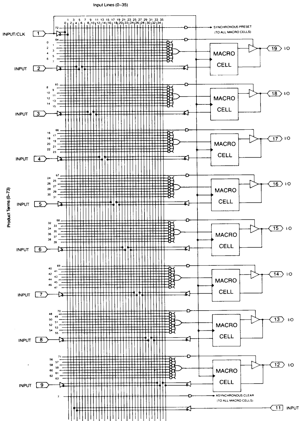
Figure 6: PEEL18CV8 Logic Array Diagram
