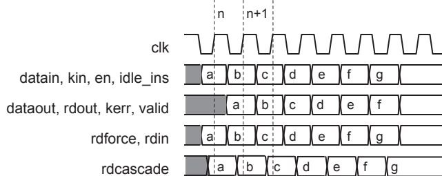
Figure 3-6. Encoder Timing Diagram—One Cycle Latency
