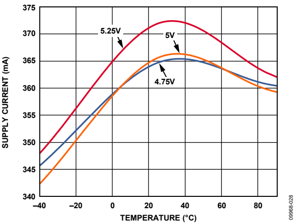
Figure 28. Supply Current vs. Temperature and Supply Voltage at 2140 MHz
