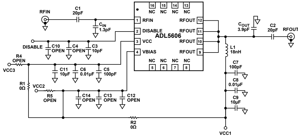
Figure 36. Evaluation Board, 2140 MHz Frequency Tuning Band
