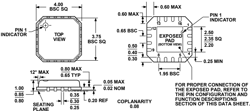
COMPLIANT TO JEDEC STANDARDS MO-220-VGGC Figure 39. 16-Lead Lead Frame Chip Scale Package [LFCSP_VQ] 4 mm × 4 mm Body, Very Thin Quad (CP-16-10) Dimensions shown in millimeters
