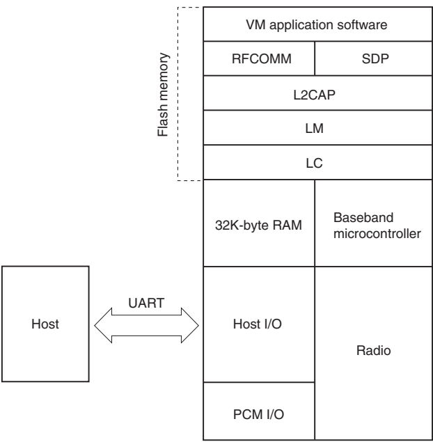
Virtual Machine Stack Configuration
