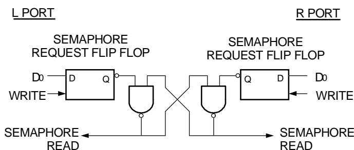
Figure 4. IDT70V16/5 Semaphore Logic
