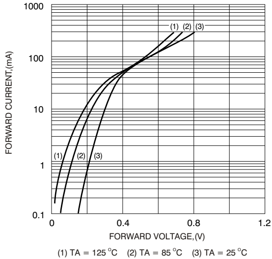
FIG.1-TYPICAL FORWARD CHARACTERISTICS
