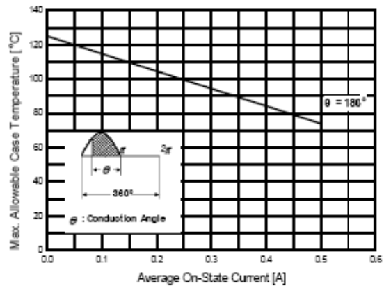
Fig 4. Thermal Response
