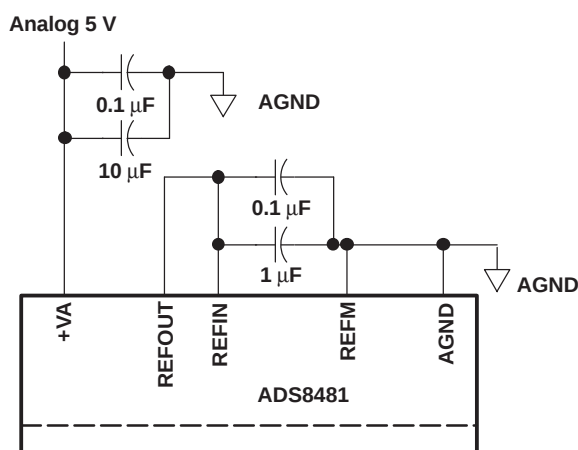
Figure 37. ADS8481 Using Internal Reference
