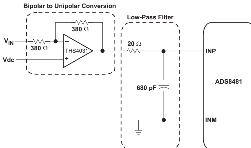
Figure 41. Input Circuit
