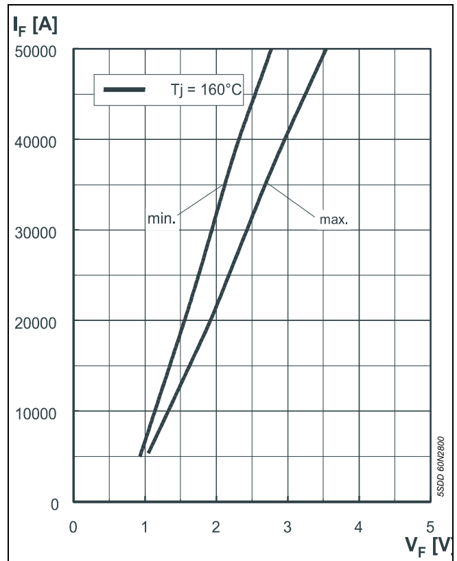
Fig. 3 On-state characteristics.
