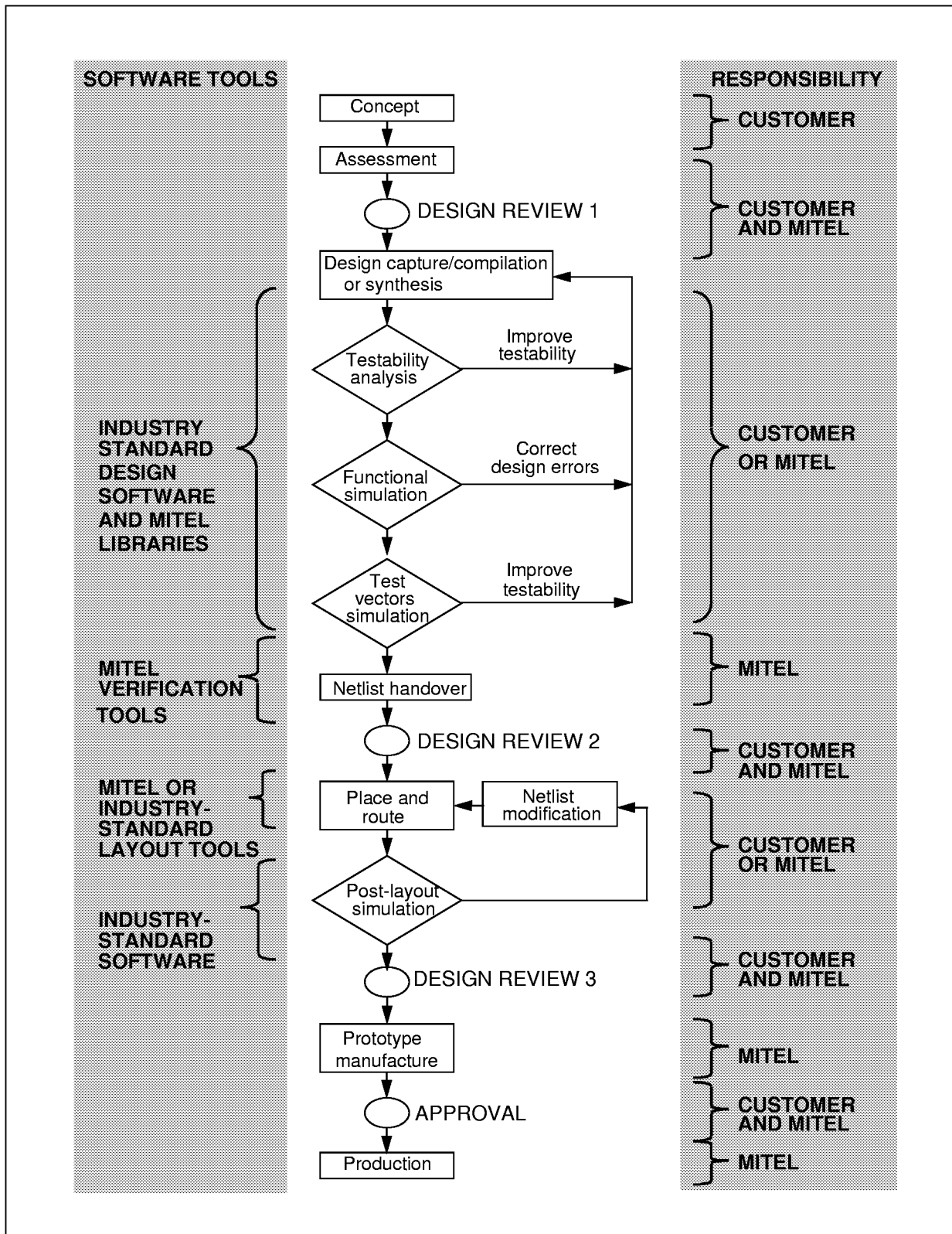
Figure 5 Design Flow
