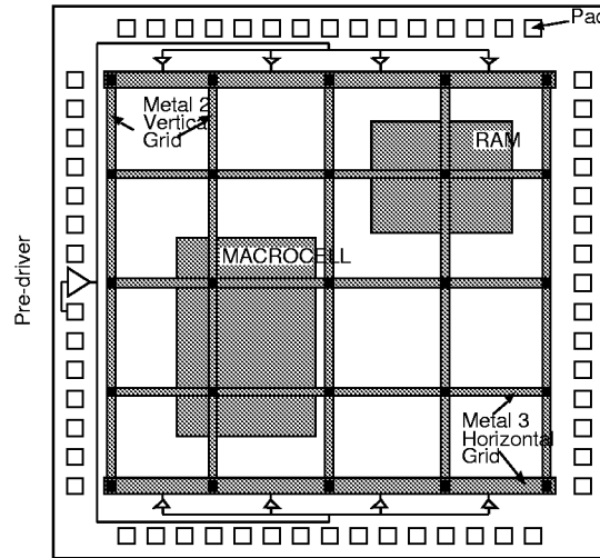
Figure 3 Example of distributed clock buffer using a grid structure
