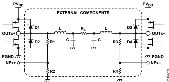
Figure 23. H-Bridge Configuration
