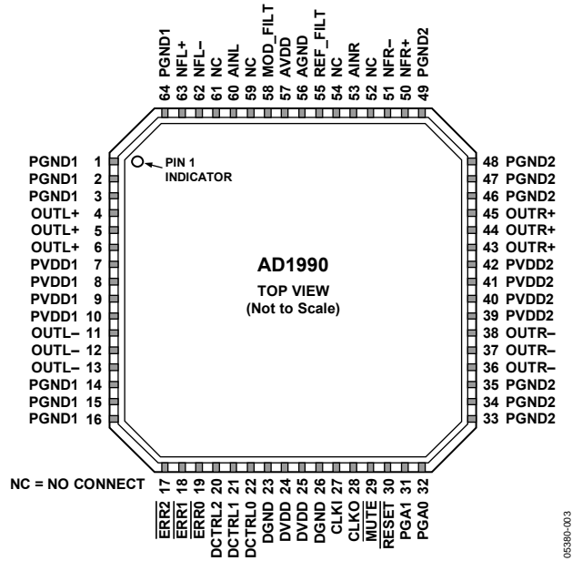
Figure 3. Pin Configuration
