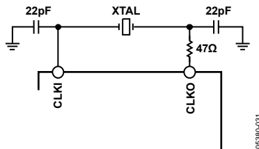
Figure 25. Crystal Connection
