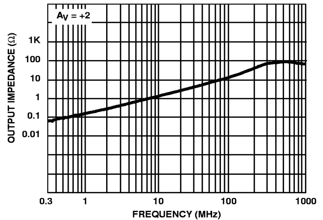
FIGURE 20. OUTPUT IMPEDANCE
