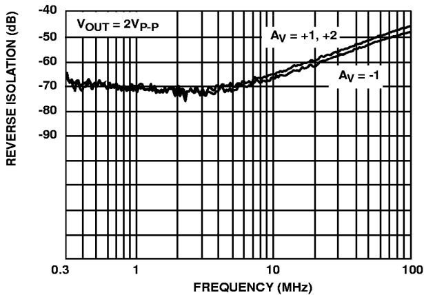
FIGURE 19. REVERSE ISOLATION
