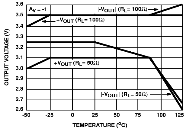
FIGURE 24. OUTPUT VOLTAGE vs TEMPERATURE
