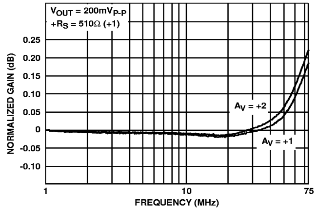
FIGURE 18. GAIN FLATNESS
