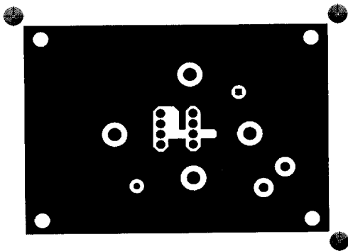
FIGURE 2B. BOTTOM LAYOUT
