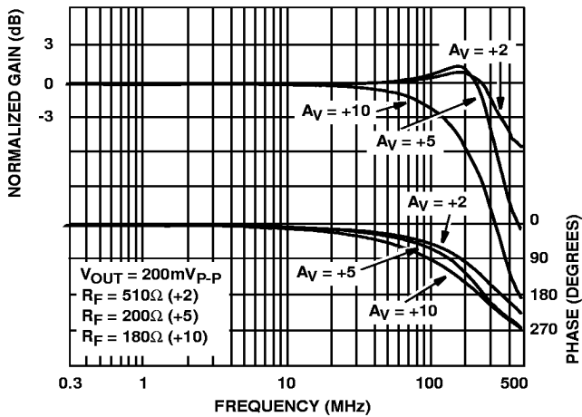
FIGURE 13. FREQUENCY RESPONSE
