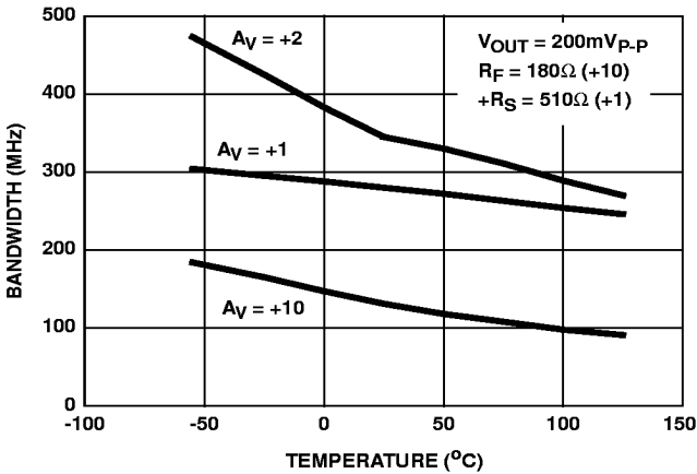
FIGURE 17. -3dB BANDWIDTH vs TEMPERATURE
