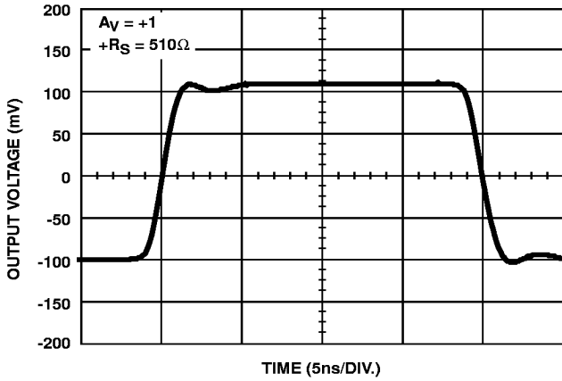
FIGURE 3. SMALL SIGNAL PULSE RESPONSE
