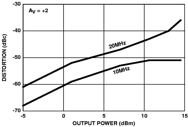
FIGURE 23. THIRD HARMONIC DISTORTION vs P_{OUT}
