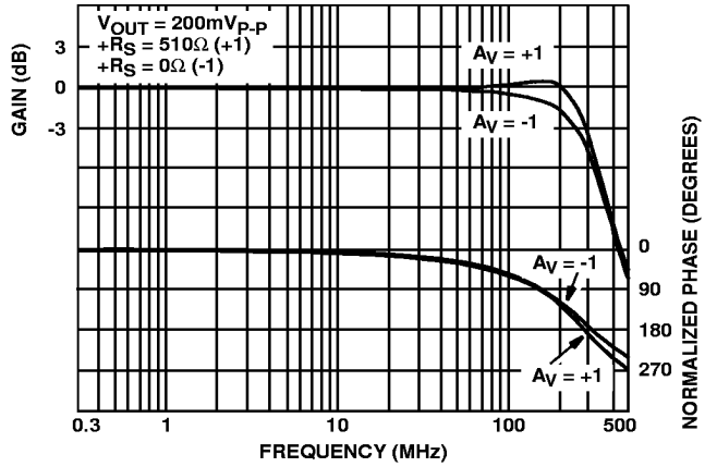
FIGURE 12. FREQUENCY RESPONSE
