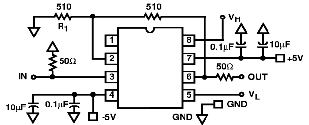
FIGURE 2C. SCHEMATIC
