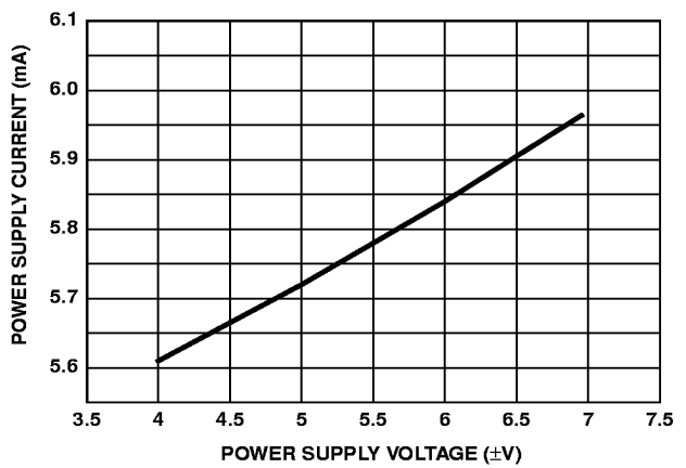
FIGURE 26. SUPPLY CURRENT vs SUPPLY VOLTAGE
