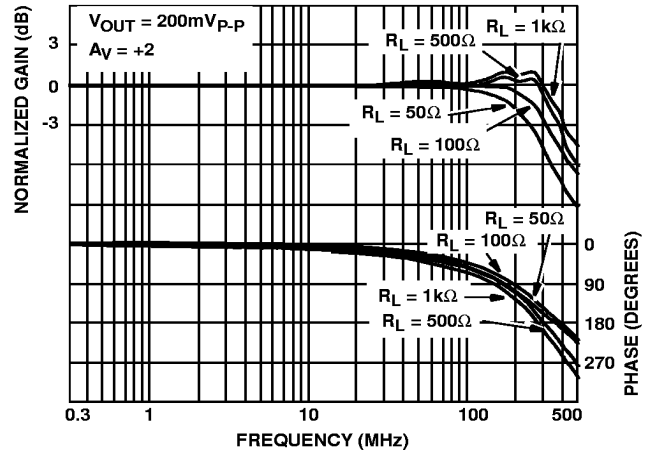
FIGURE 16. FREQUENCY RESPONSE FOR VARIOUS LOAD RESISTORS
