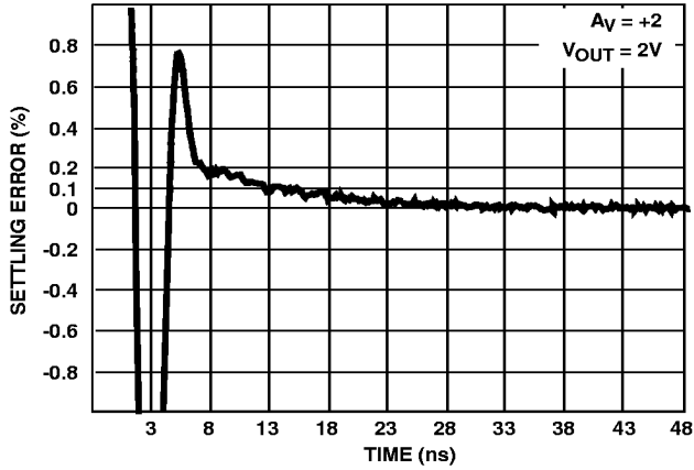
FIGURE 21. SETTLING RESPONSE
