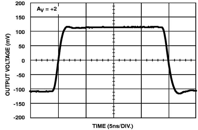
FIGURE 6. SMALL SIGNAL PULSE RESPONSE
