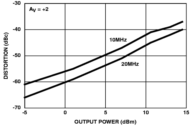
FIGURE 22. SECOND HARMONIC DISTORTION vs P_{OUT}
