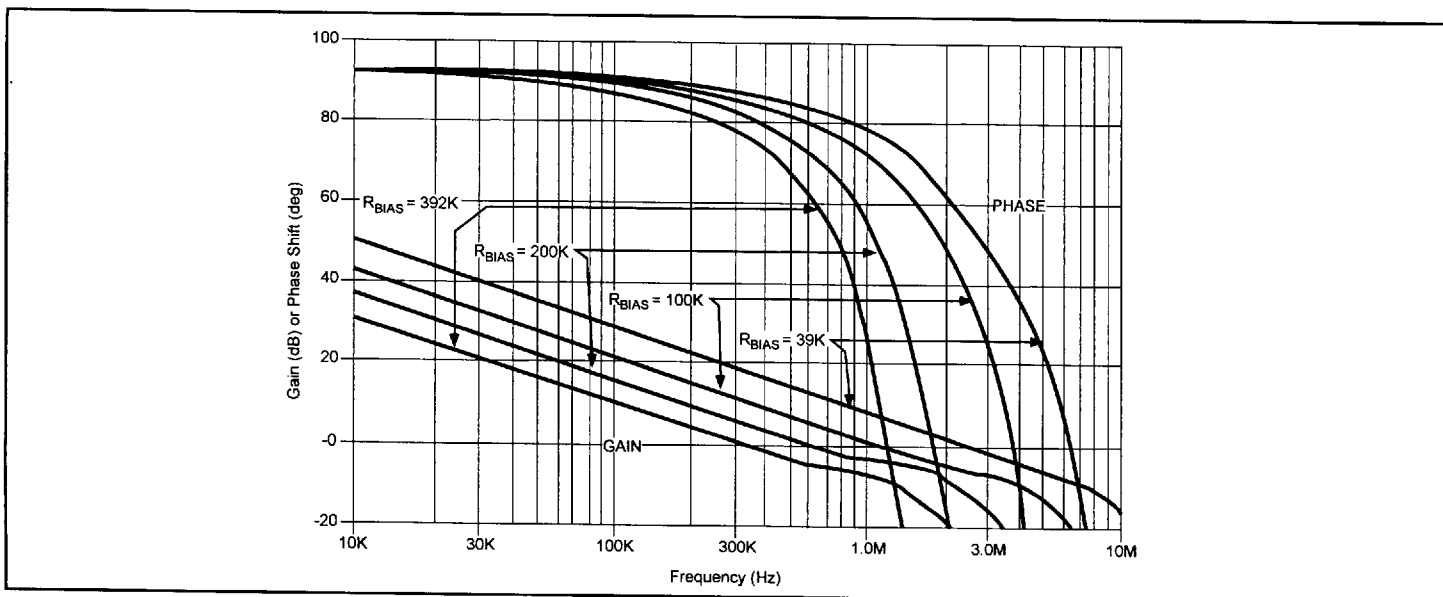
ERROR AMPLIFIER GBW VERSUS R_{BIAS}
