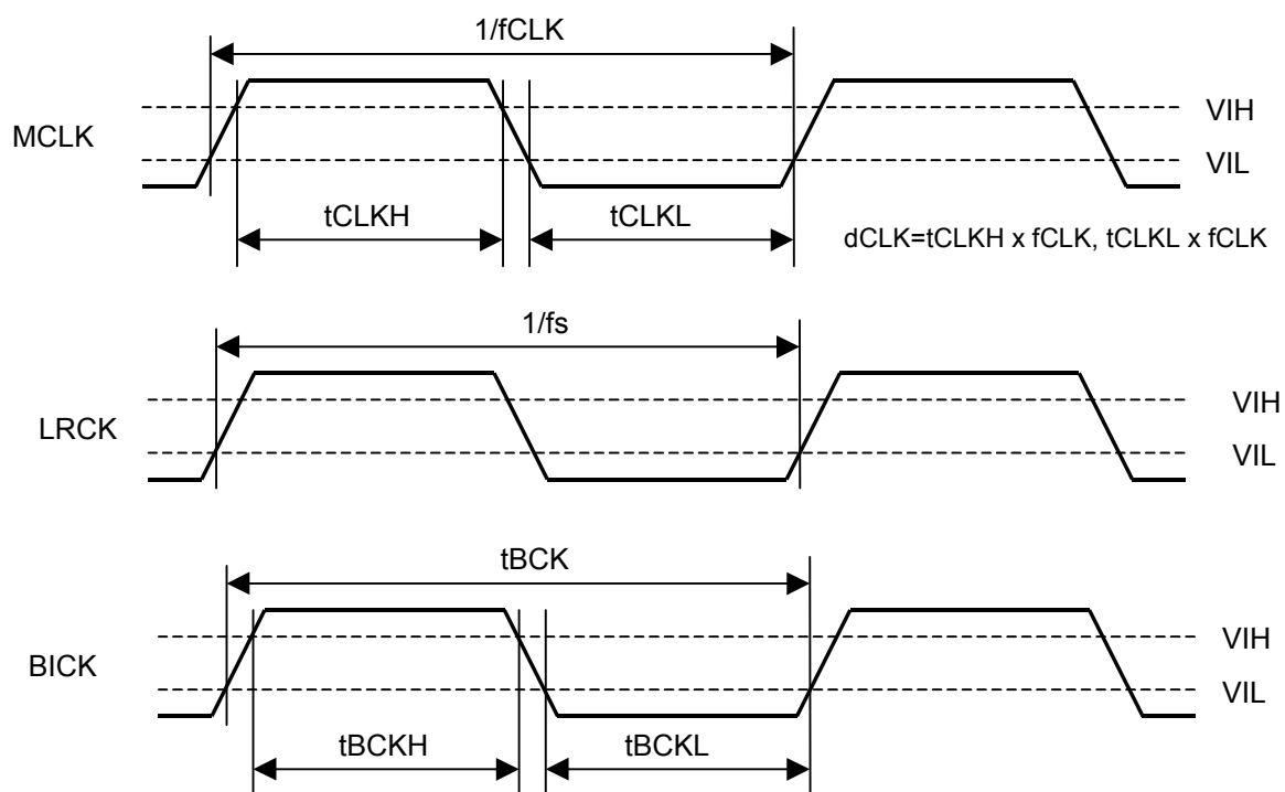
Figure 1. Clock Timing
