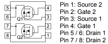
H4946DS Symbol & Pin Assignment
